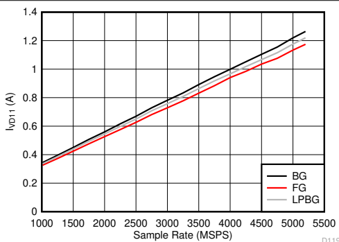
Figure 5-133. Dual Channel Mode: I_{VD11} vs Sample Rate
