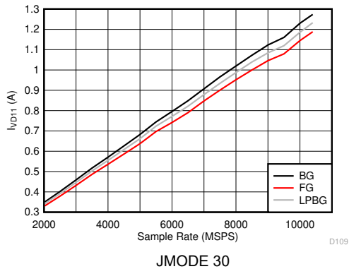
Figure 5-125. DES Mode: I_{VD11} vs Sample Rate
