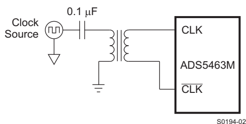
Figure 19. Differential Clock
