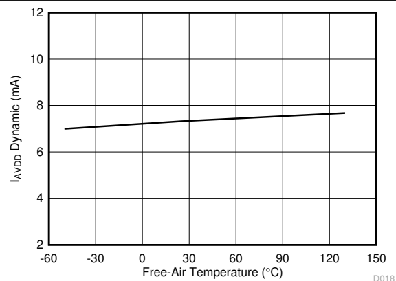
Figure 6-9. Analog Supply Current vs Temperature
