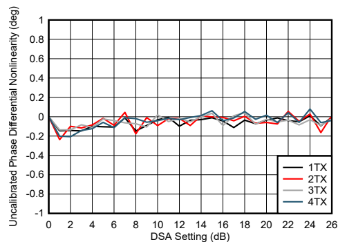
Figure 5-240. TX DSA Uncalibrated Phase Differential Nonlinearity
