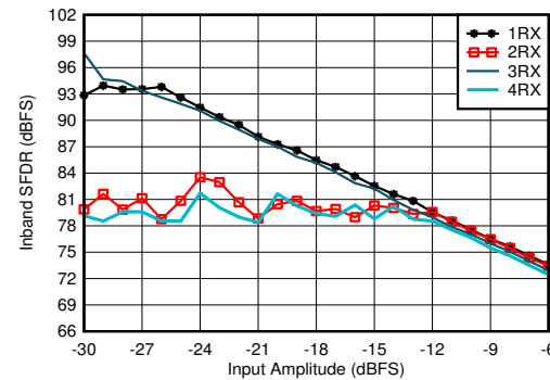
Figure 5-411. RX In-Band SFDR ( \pm 400\text{ MHz} ) vs Input Amplitude and Channel at 4.9 GHz
