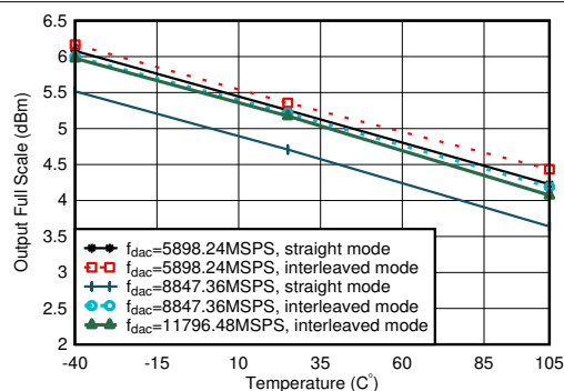
Figure 5-2. TX Output Fullscale vs Temperature
