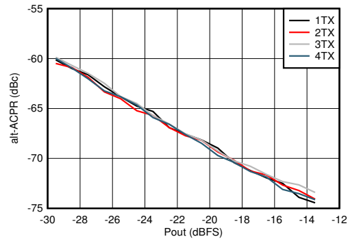
Figure 5-105. TX 20-MHz LTE alt-ACPR vs Digital Level at 2.6 GHz
