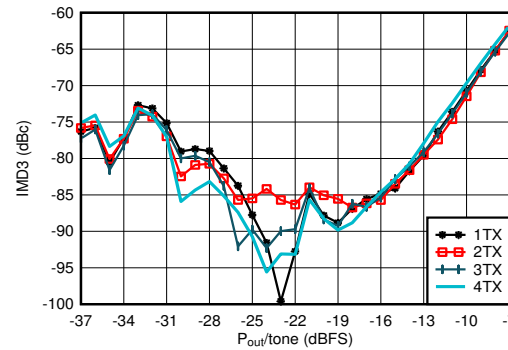
Figure 5-28. TX IMD3 vs Digital Level at 0.85 GHz
