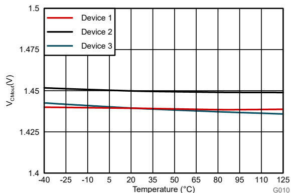
Figure 6-32. Output Common-Mode Voltage vs Temperature
