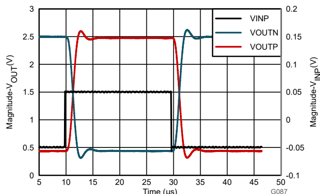
Figure 8-4. Step Response of the AMC0x02D
