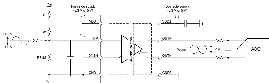
Typical Application
