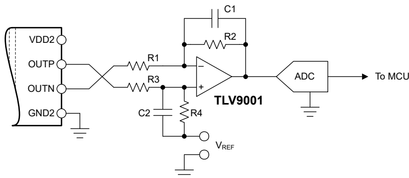
Figure 8-3. Connecting the AMC0x30D Output to a Single-Ended Input ADC
