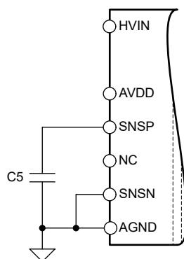
Figure 8-2. Input Filter
