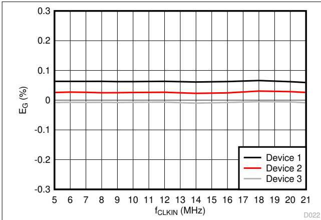
Figure 6-12. Gain Error vs Input Clock Frequency
