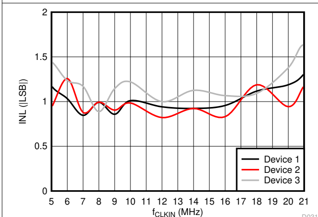
Figure 6-16. Integral Nonlinearity vs Input Clock Frequency
