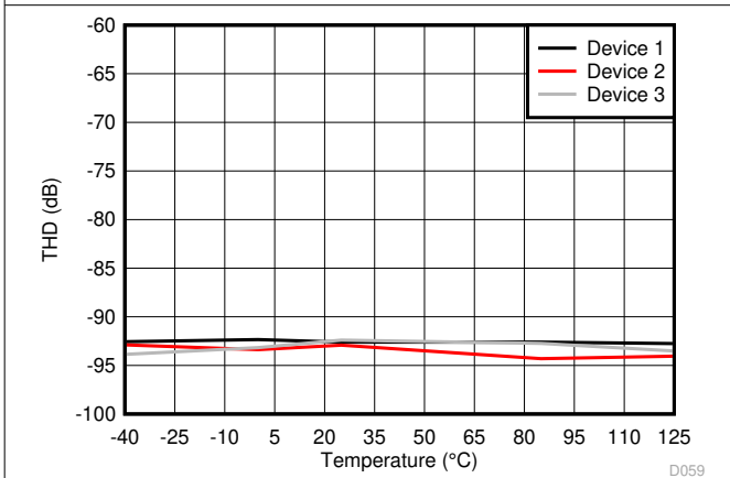
Figure 6-28. Total Harmonic Distortion vs Temperature
