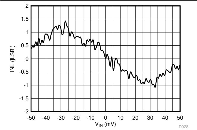
Figure 6-15. Integral Nonlinearity vs Input Voltage
