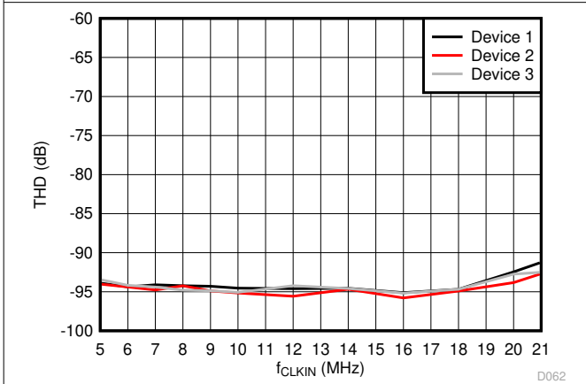
Figure 6-26. Total Harmonic Distortion vs Input Clock Frequency
