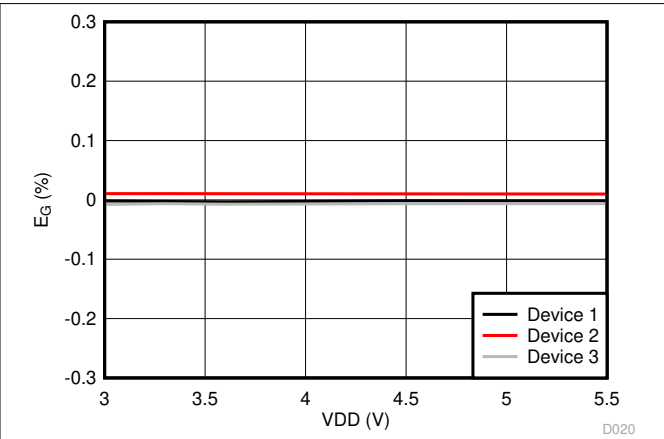
Figure 6-13. Gain Error vs Supply Voltage
