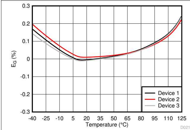
Figure 6-14. Gain Error vs Temperature
