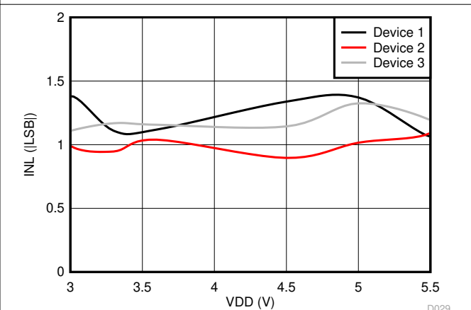
Figure 6-17. Integral Nonlinearity vs Supply Voltage
