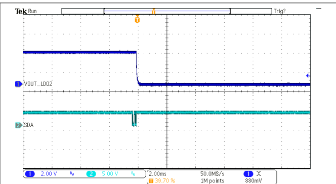
Figure 8-27. LDO2 Disable (No load)
