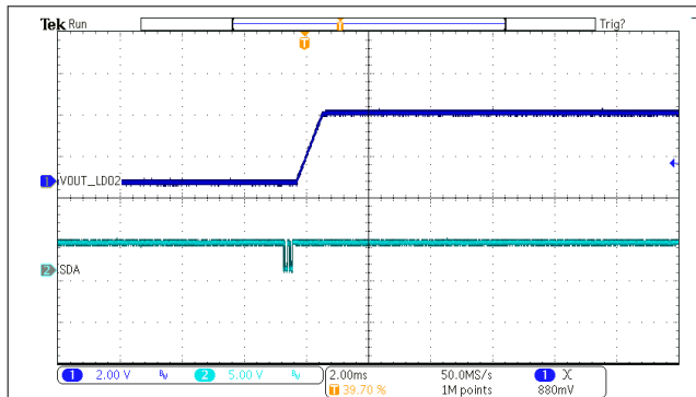
Figure 8-26. LDO2 Enable (No load)
