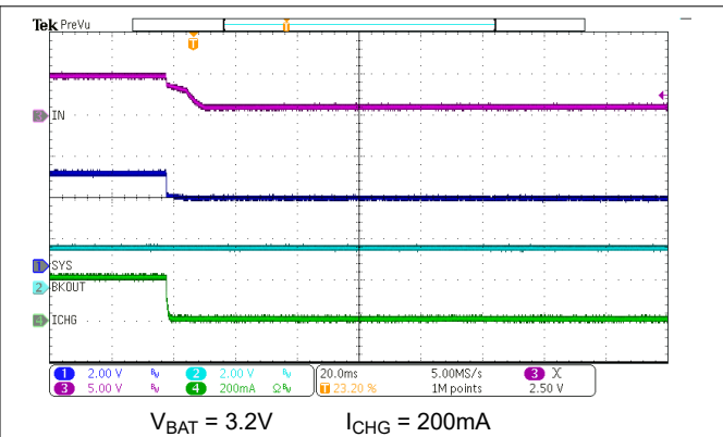
Figure 8-3. Adapter Unplug with Charge Enabled
