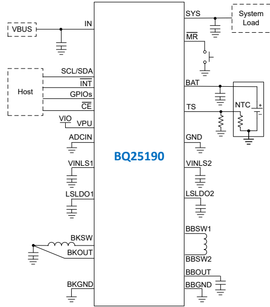
Simplified Schematic
