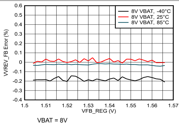
Figure 6-4. Reverse Feedback Voltage Accuracy (at different temperatures)
