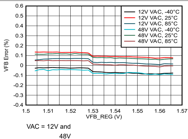
Figure 6-3. Forward Feedback Voltage Accuracy (at different temperatures)
