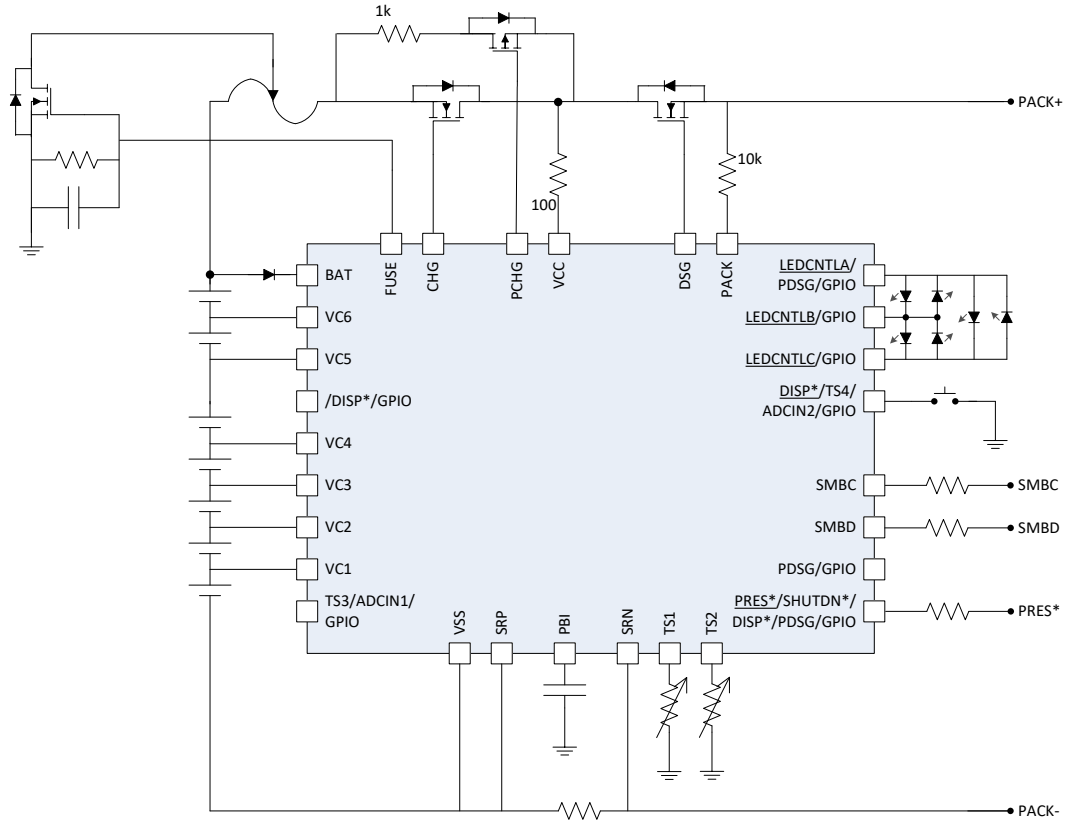
Simplified Schematic
