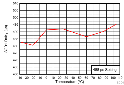
Figure 5-12. Short Circuit Discharge 1 Delay Time vs Temperature
