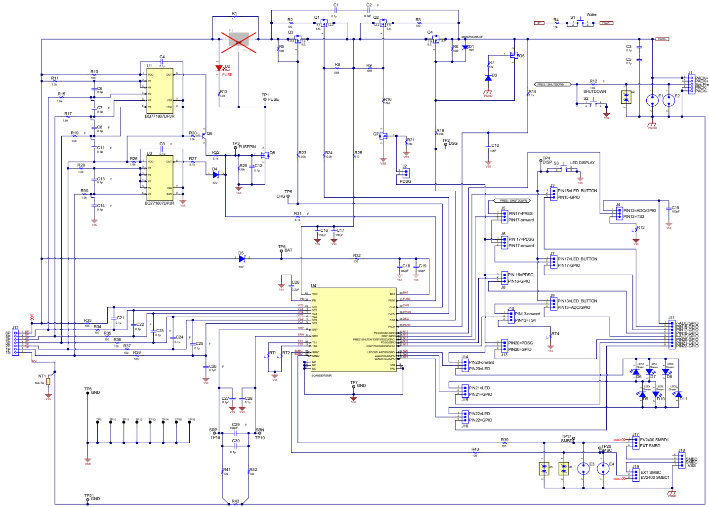
Figure 7-1. BQ40Z80EVM Gauge and Protector Schematic
