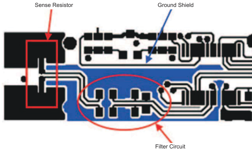
Figure 7-6. Sense Resistor, Ground Shield, and Filter Circuit Layout
