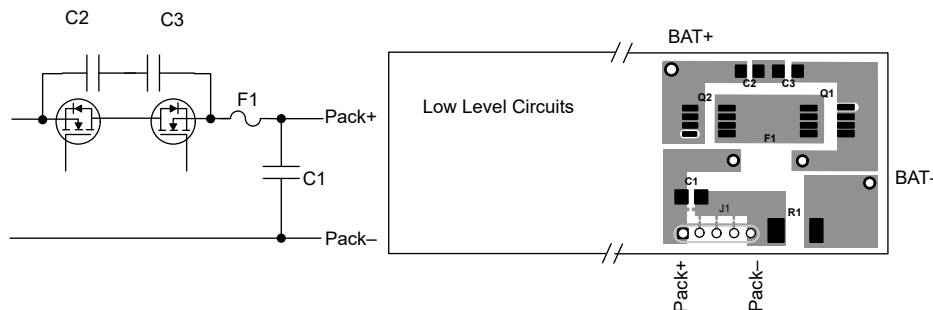
Figure 7-7. Wide Copper Traces Lower the Inductance of Bypass Capacitors C1, C2, and C3
