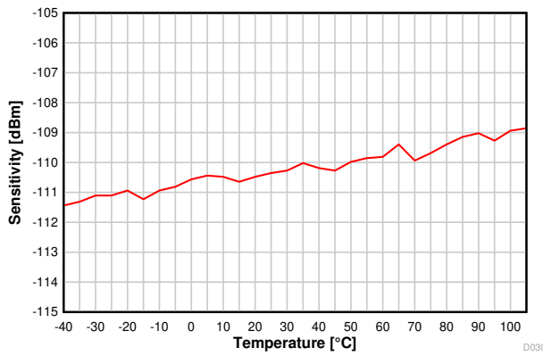
Figure 7-15. Sensitivity vs Temperature (50kbps, 868.3MHz)
