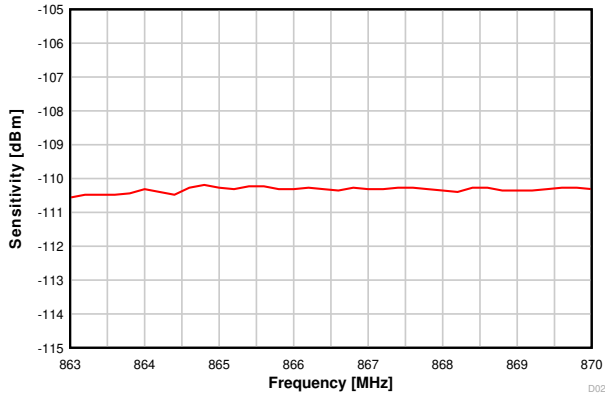
Figure 7-13. Sensitivity vs Frequency (50kbps, 868MHz)
