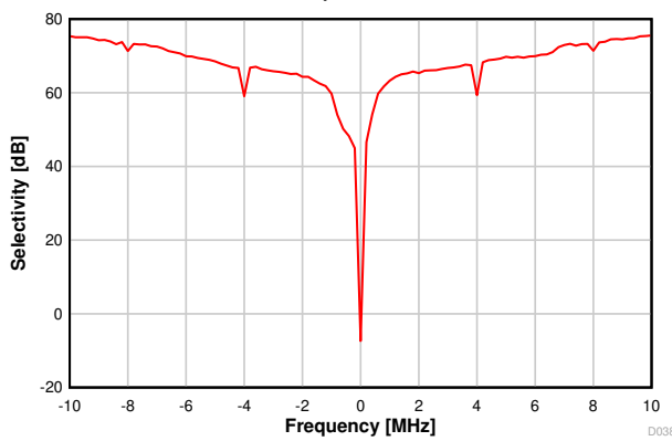
Figure 7-17. Selectivity vs Frequency Offset (50kbps, 868.3MHz)
