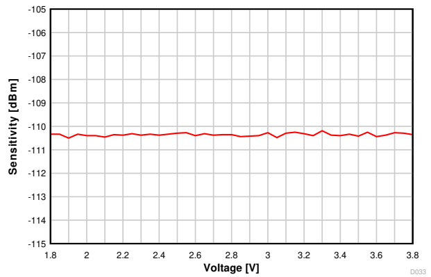
Figure 7-16. Sensitivity vs Supply Voltage (VDD5) (50kbps, 868.3MHz)
