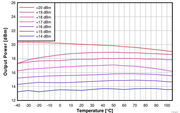
Figure 7-22. Output Power vs Temperature (50kbps, 915MHz)
