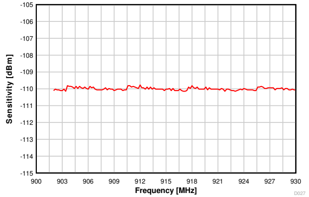
Figure 7-14. Sensitivity vs Frequency (50kbps, 915MHz)
