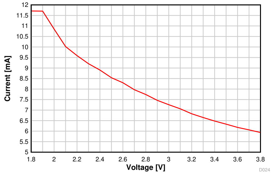
Figure 8-16. TX Current vs. Supply Voltage (VDD5) (BLE 1 Mbps, 2.44 GHz)
