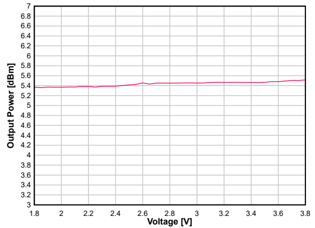
Figure 8-19. Output Power vs. Supply Voltage (VDDS) (BLE 1 Mbps, 2.44 GHz, +5dBm)
