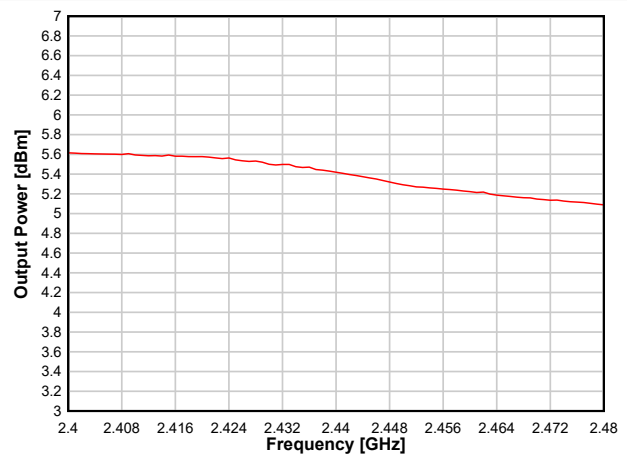
Figure 8-21. Output Power vs. Frequency (BLE 1 Mbps, +5dBm)
