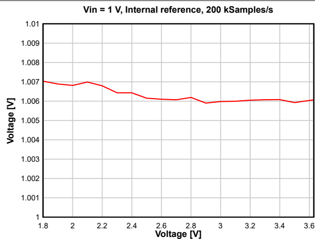
Figure 8-30. ADC Accuracy vs. Supply Voltage (VDD)
