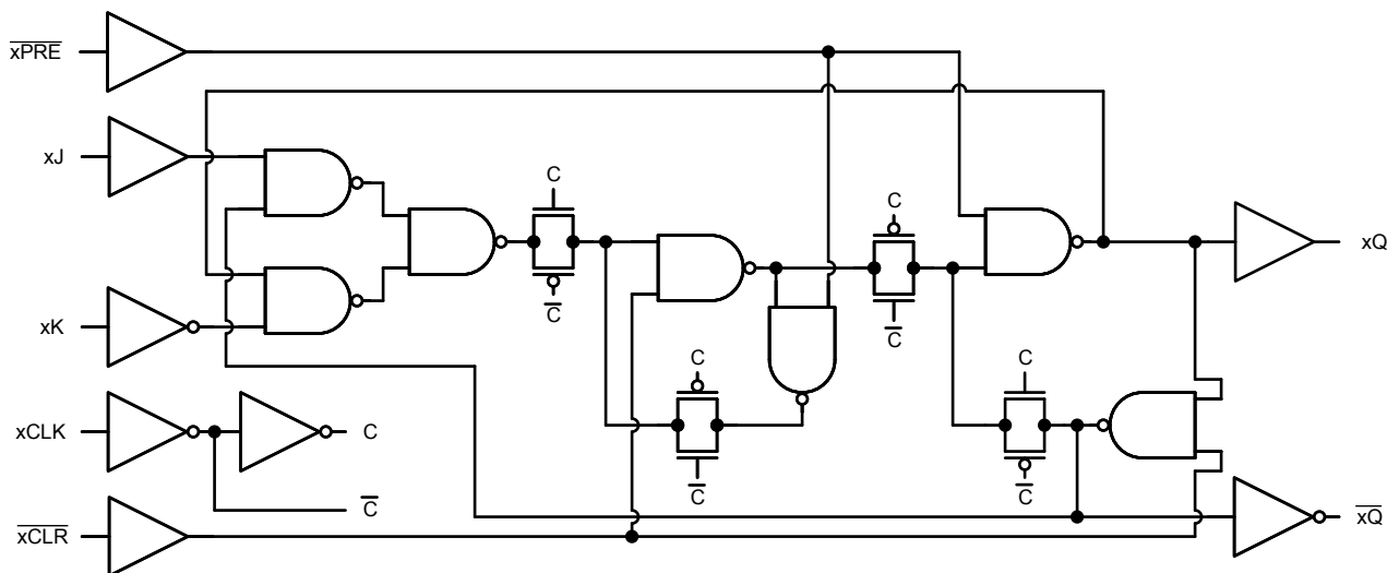
Functional Diagram
