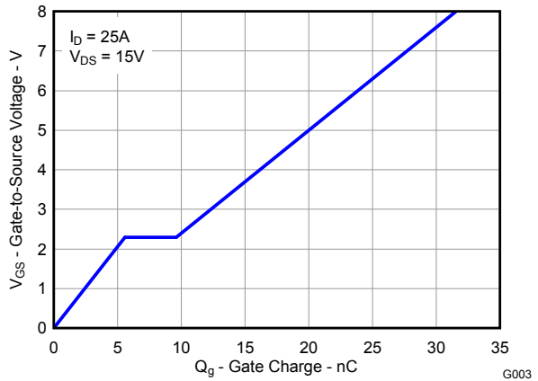
Figure 4. Gate Charge
