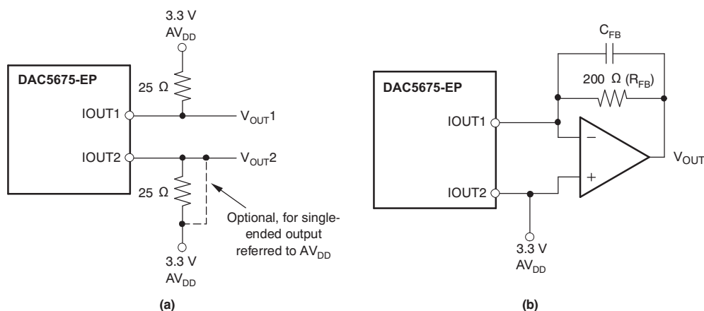
Figure 24. Output Configurations
