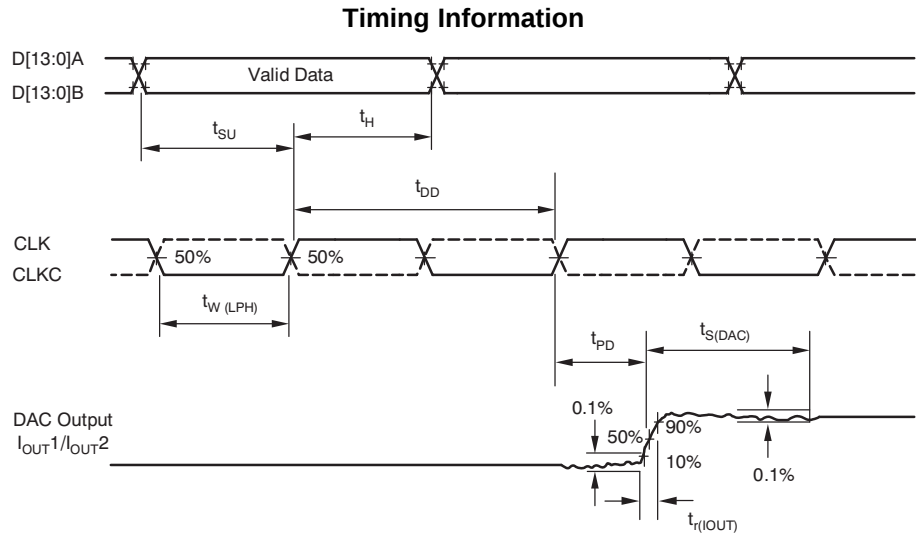
Figure 1. Timing Diagram
