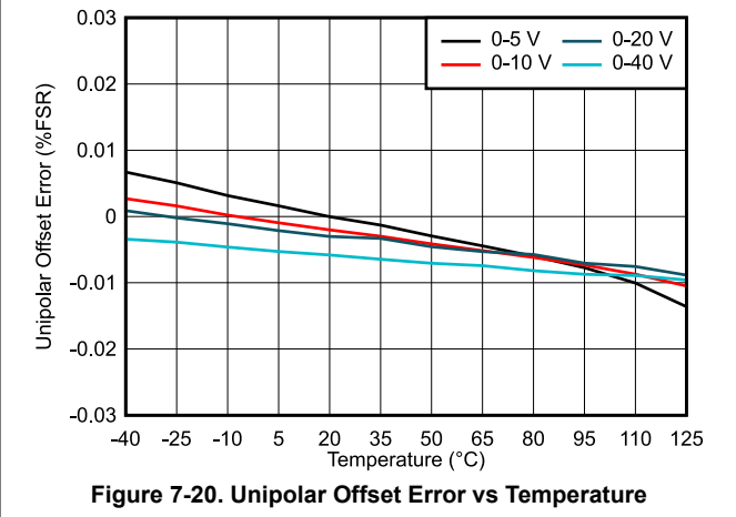
Figure 7-20. Unipolar Offset Error vs Temperature
