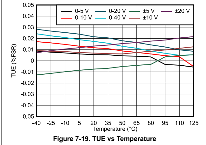
Figure 7-19. TUE vs Temperature
