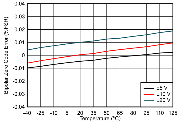
Figure 7-22. Bipolar Zero Code Error vs Temperature
