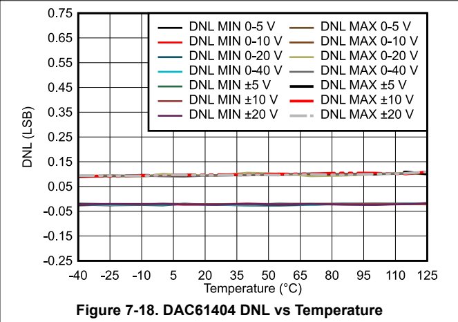
Figure 7-18. DAC61404 DNL vs Temperature
