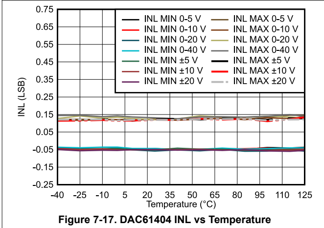
Figure 7-17. DAC61404 INL vs Temperature
