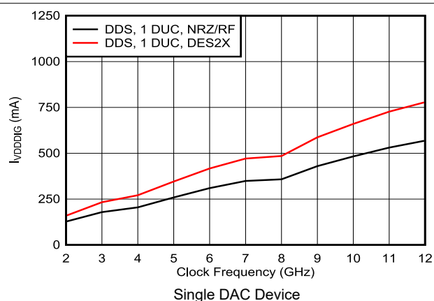
Figure 6-59. VDDDIG Current vs Clock Frequency and DAC Mode
