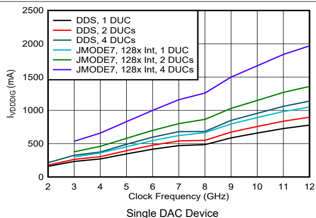
Figure 6-57. VDDDIG Current vs Clock Frequency and Digital Mode
