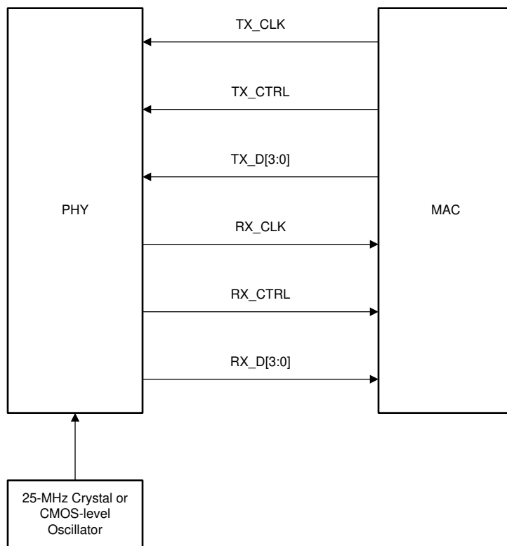
Figure 7-13. RGMII Connections
