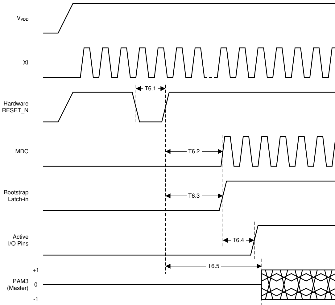
Figure 6-2. Reset Timing
