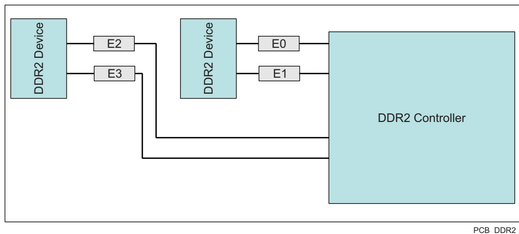
Figure 8-56. DQS and DQ Routing and Topology
