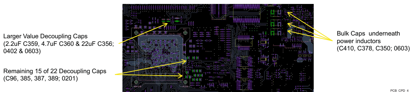
Figure 8-24. vdd_mpu routing and cap placements [Bottom Layer]
