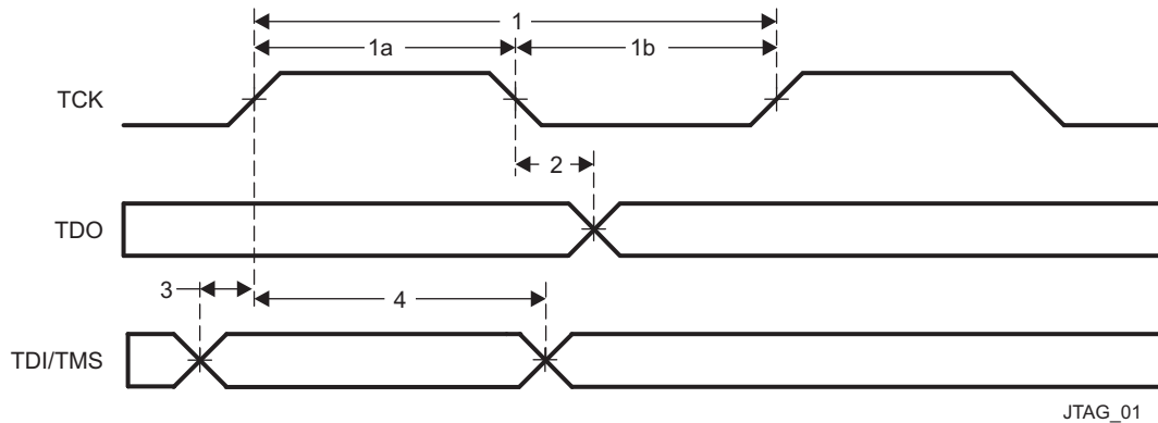
Figure 7-94. JTAG Timing
