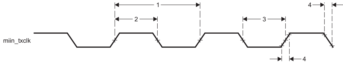
Figure 7-53. Clock Timing (GMAC Transmit) - MII operation
