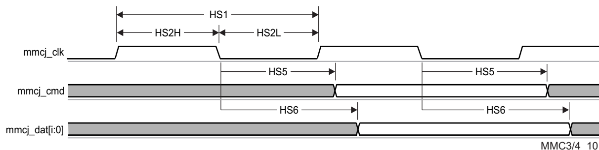
Figure 7-86. MMC/SD/SDIOj in - High Speed - Transmitter Mode
