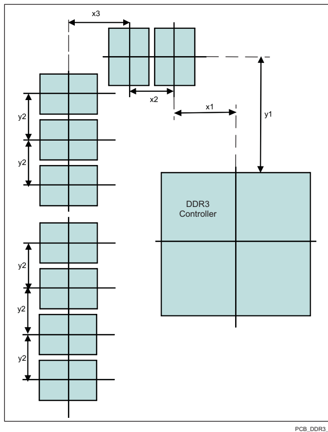
Figure 8-60. Placement Specifications
