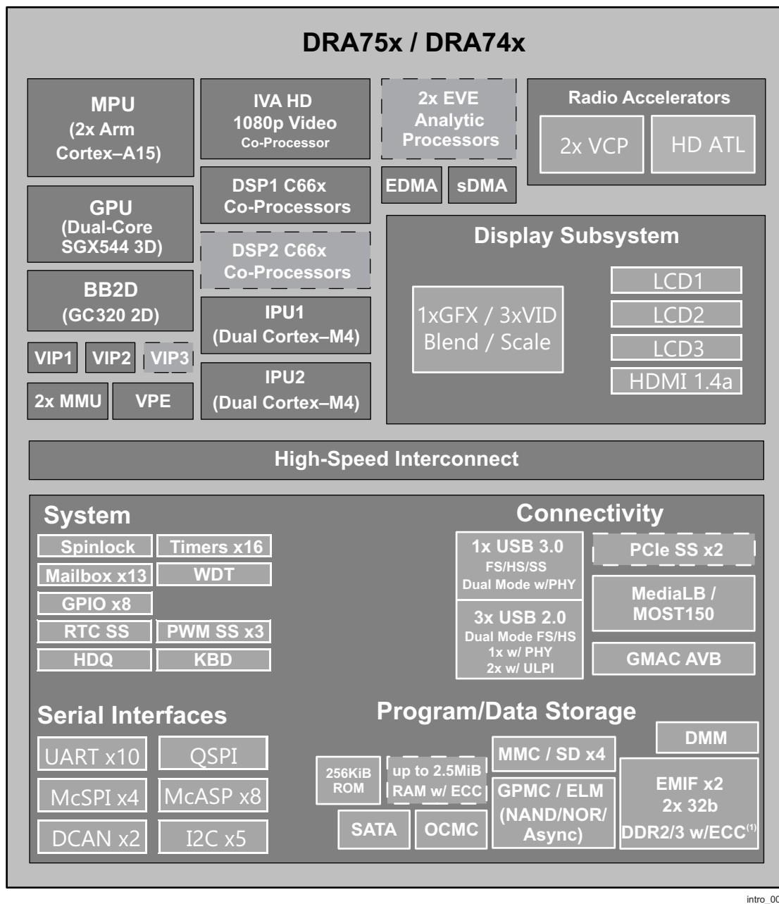
Figure 1-1. DRA75x, DRA74x Block Diagram
