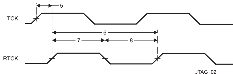
Figure 7-95. JTAG With RTCK Timing
