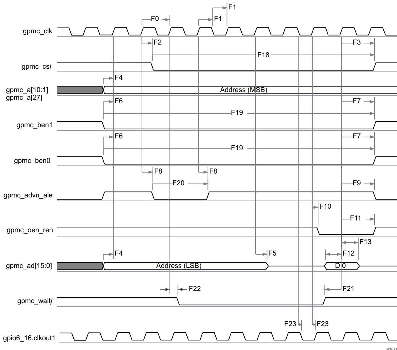
Figure 7-7. GPMC / Multiplexed 16bits NOR Flash - Synchronous Single Read - (GpmcFCLKDivider = 0) (1)(2)
