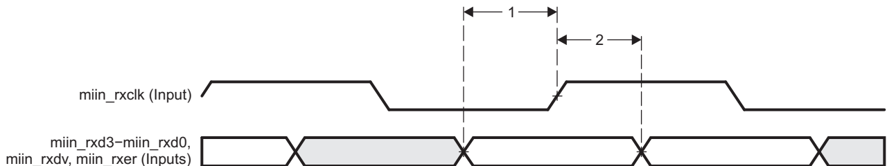
Figure 7-54. GMAC Receive Interface Timing MII operation
