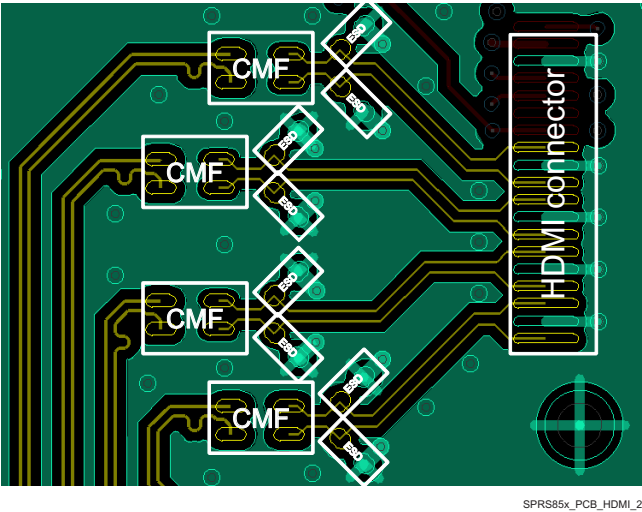
Figure 8-43. HDMI Placement Diagram
