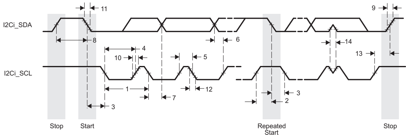
Figure 7-23. I2C Receive Timing
