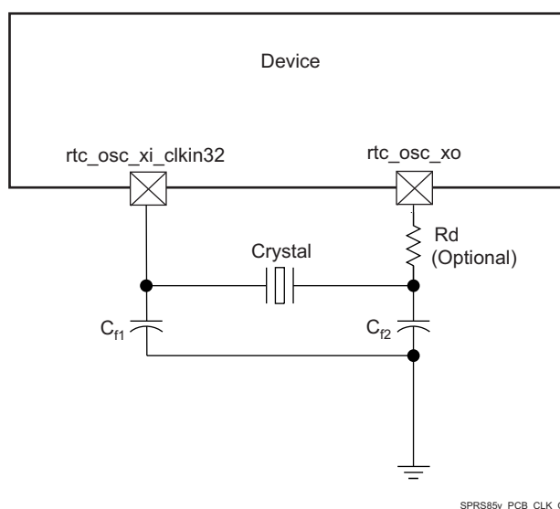
Figure 8-47. Grounding Scheme for Low-Frequency Clock
