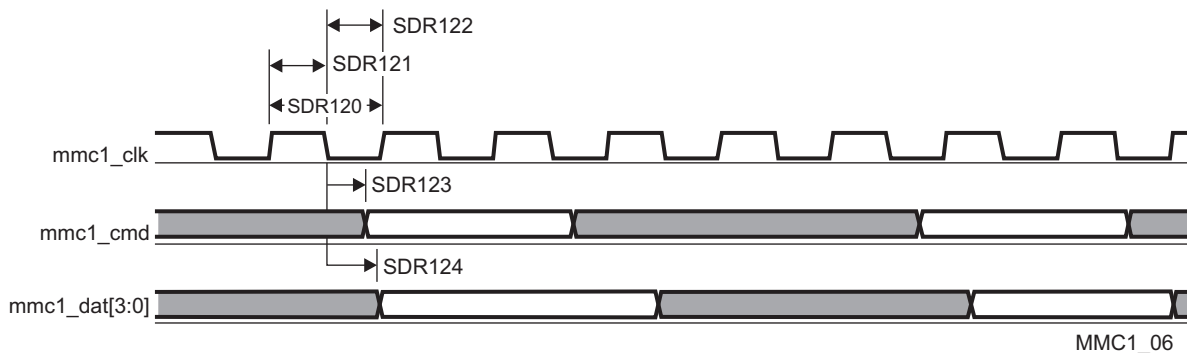
Figure 7-67. MMC/SD/SDIO in - High Speed SDR12 - Transmitter Mode
