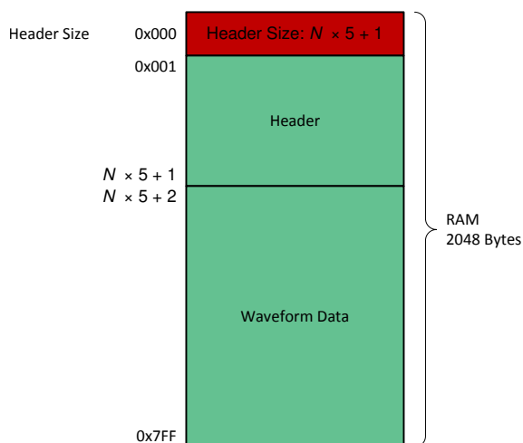
Figure 7-5. RAM Structure
