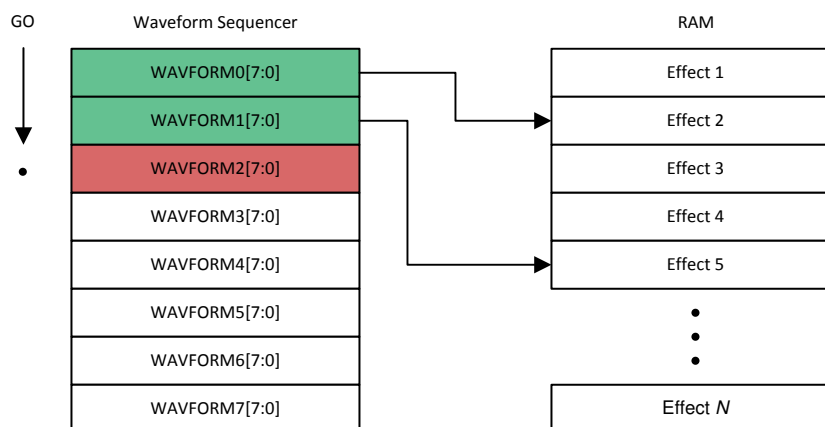
Figure 7-9. Waveform Sequencer
