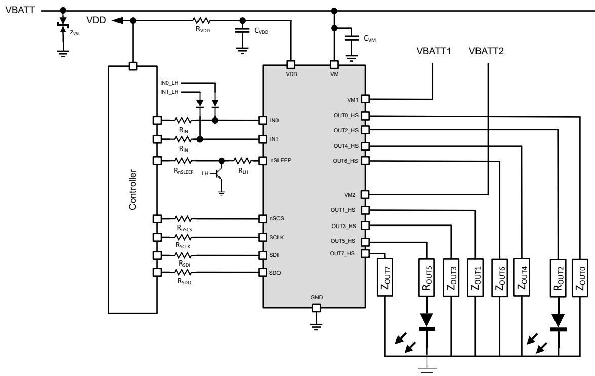
Figure 8-2. Application Schematic
