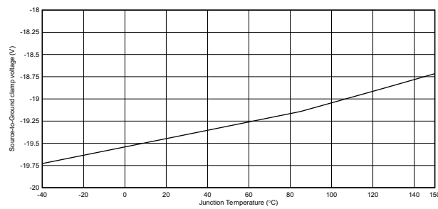
Figure 6-6. Source-to-Ground Clamp Voltage
