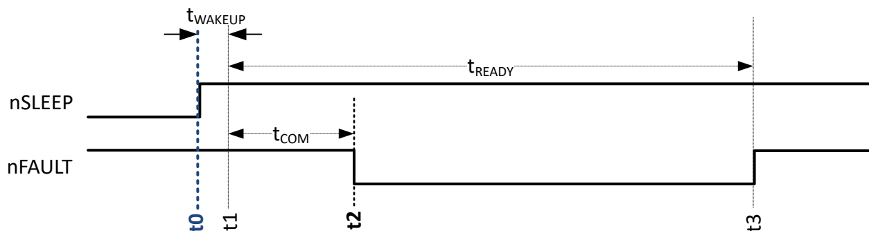
Figure 6-4. Wake-up from SLEEP State to STANDBY State without ACK Pulse
