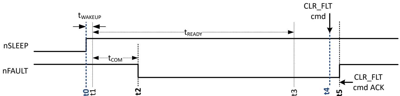
Figure 6-8. Wake-up from SLEEP State to STANDBY State
