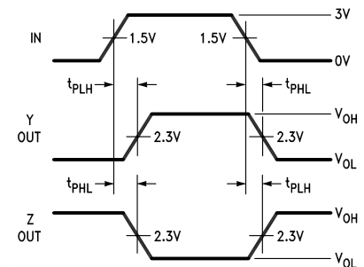
Figure 6. Driver Differential Output Delay and Transition Times (2)(3)
