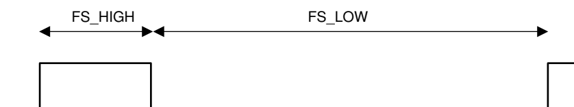
Figure 7-17. Internal FrameSync
