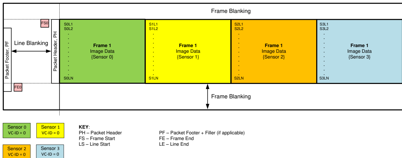
Figure 7-21. Line-Concatenated Format
