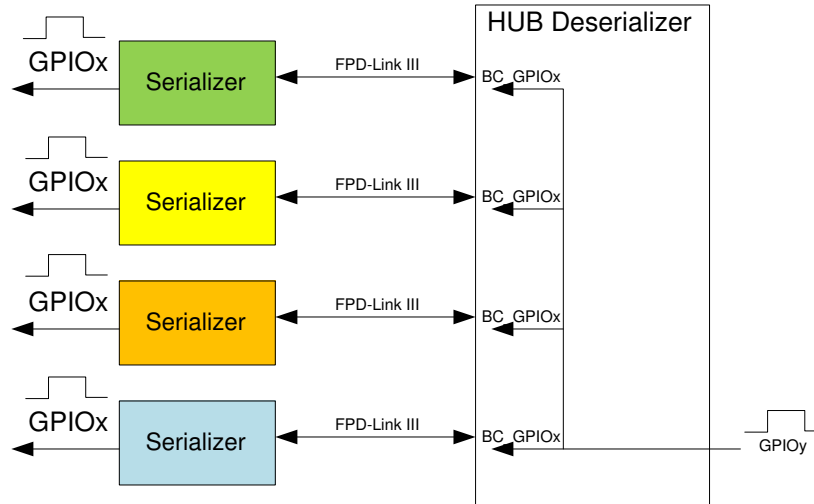
Figure 7-16. External FrameSync
