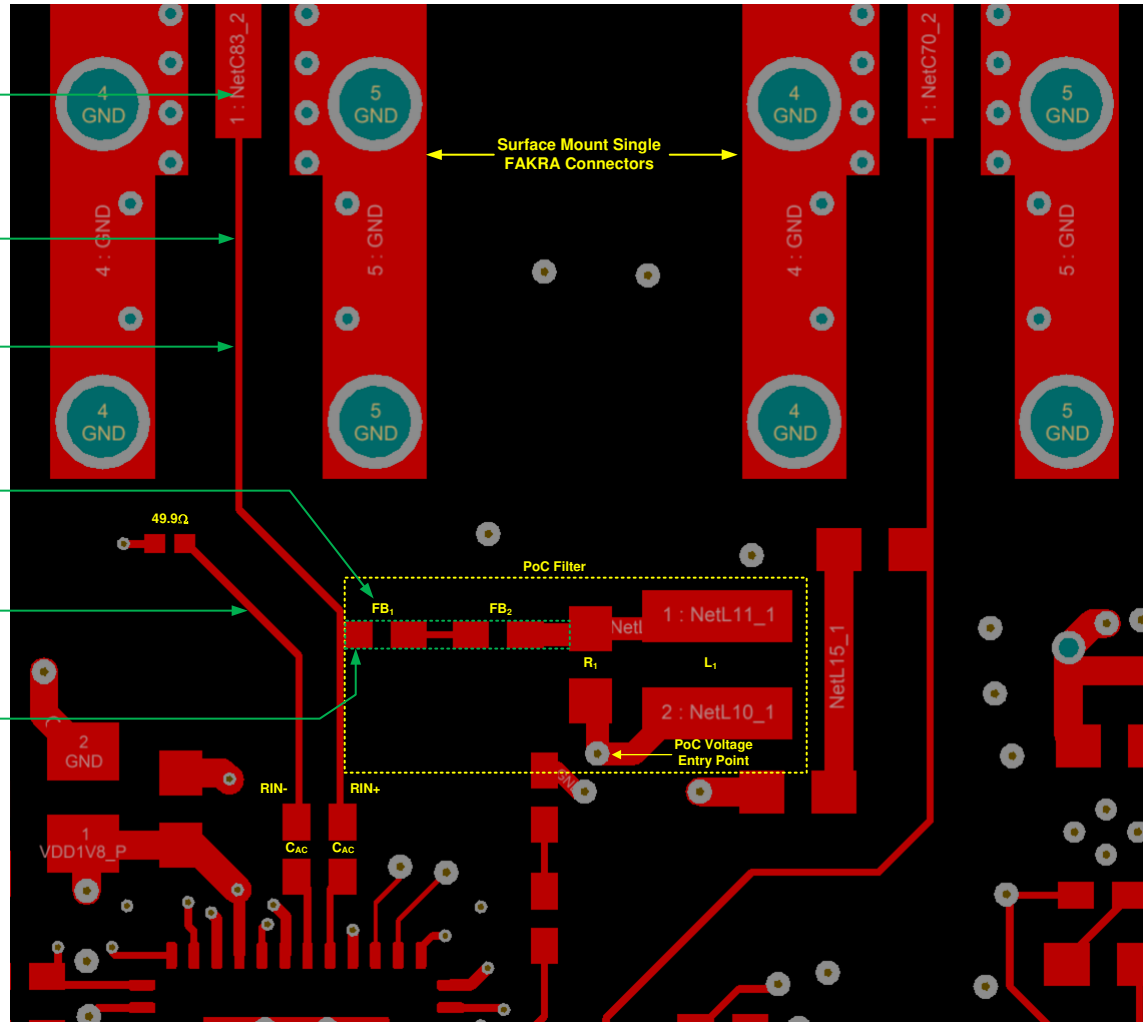
Figure 8-22. Example Routing of FPD-Link III Traces to a Single Mini-Fakra Connector and PoC Components
