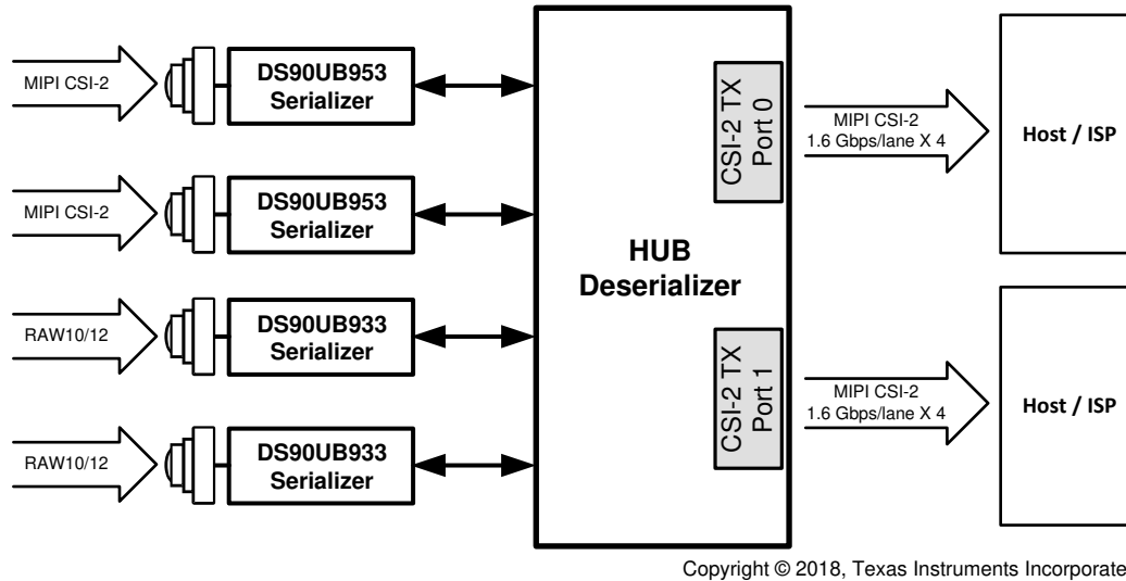
Figure 8-17. Two DS90UB933-Q1 and Two DS90UB953-Q1 Sensor Data Onto CSI-2 Over 2 Ports
