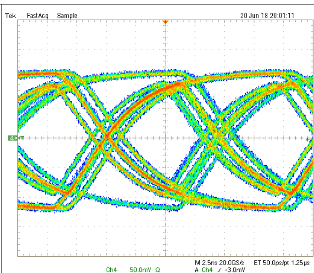
Figure 6-12. Typical 50 Mbps Back Channel Output Waveform
