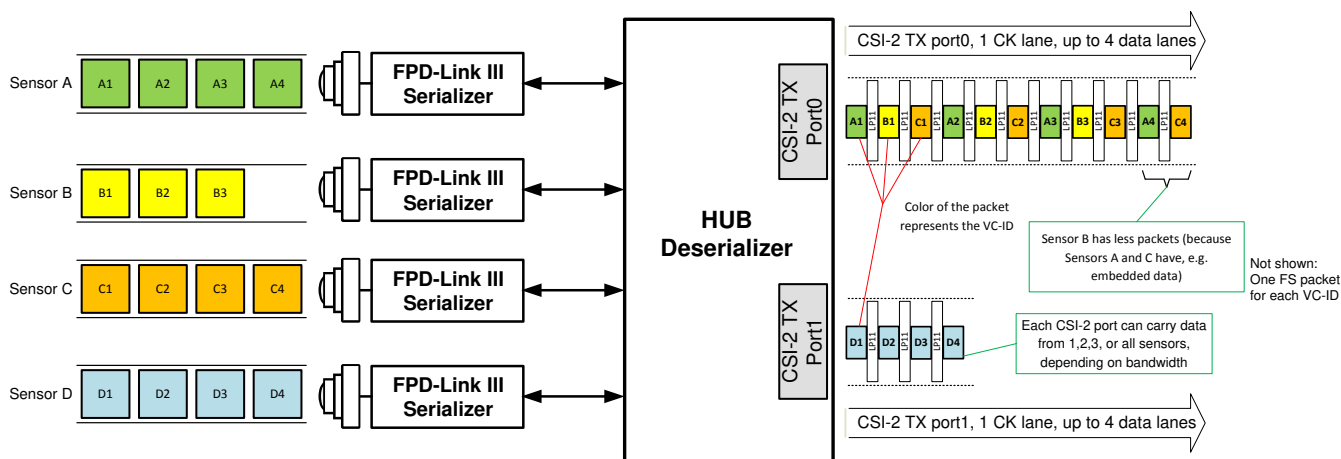
Figure 7-14. Four Sensor Data onto CSI-2 With Virtual Channels (VC-ID) With Different Frame Size
