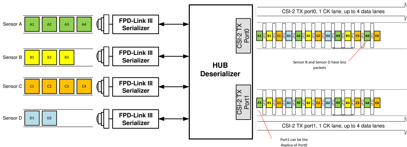
Figure 7-15. Four Sensor Data onto 1xCSI-2 Replicated With Virtual Channels (VC-ID) With Different Frame Size
