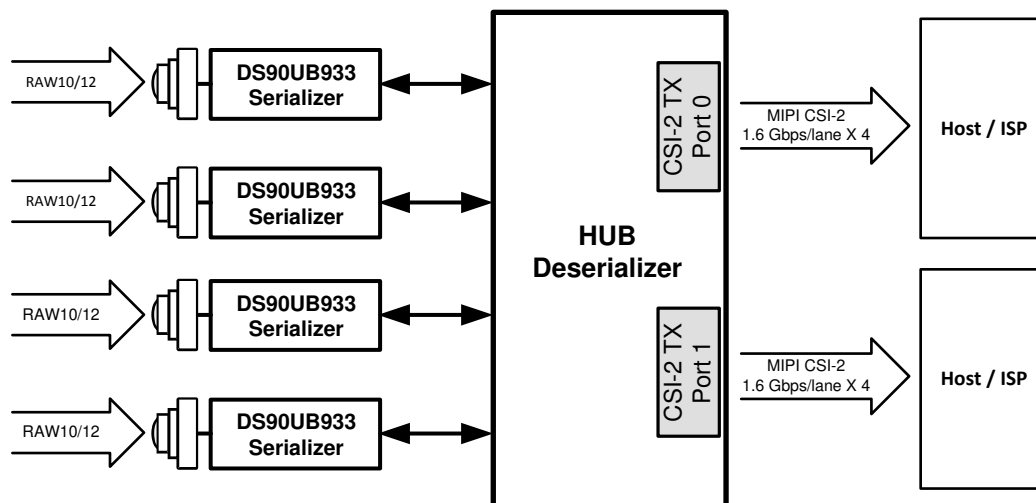
Figure 8-15. Four DS90UB933-Q1 Sensor Data Onto CSI-2 Over 2 Ports
