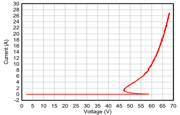
Figure 5-14. Negative TLP Curve
