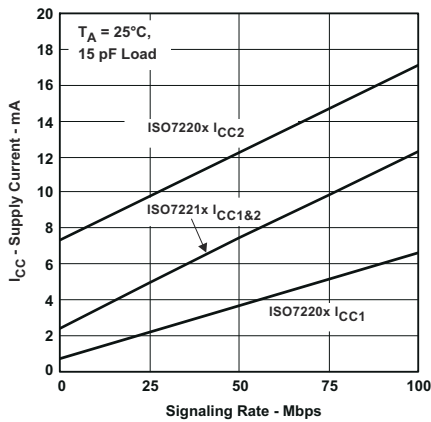
Figure 5-1. 3.3-V RMS Supply Current vs Signaling Rate (Mbps)
