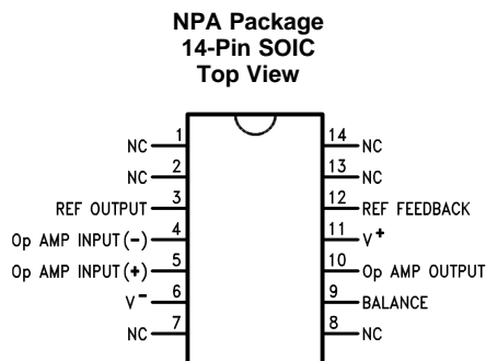
Pin Functions — 14-Pin SOIC
