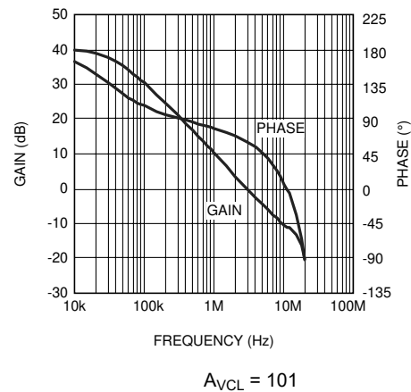
Figure 5-6. Error Amplifier Gain and Phase
