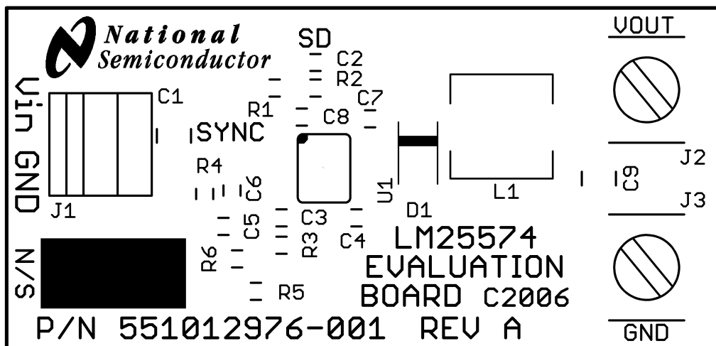
Figure 7-14. Silkscreen
