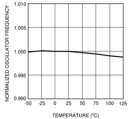
Figure 5-2. Oscillator Frequency vs Temperature
