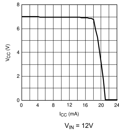
Figure 5-4. V_{CC} vs I_{CC}
