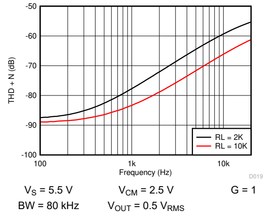
Figure 6-13. THD + N vs Frequency
