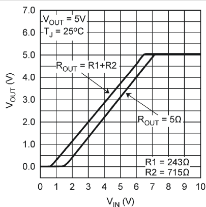
Figure 6-7. Line Regulation (Legacy Chip)
