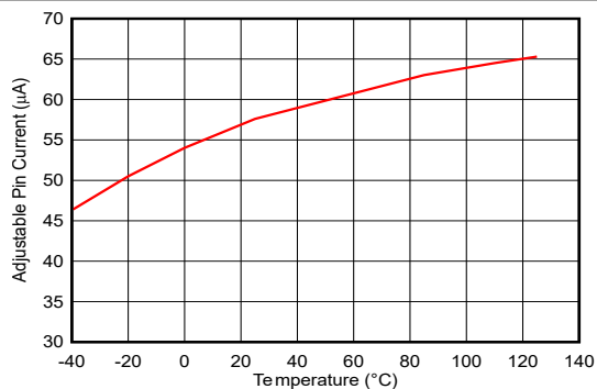
Figure 5-1. Change in Adjustment Current Over Temperature (Legacy Chip)
