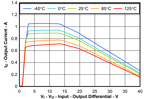
Figure 5-10. Minimum Operating Current vs Input-Output Differential Voltage (New Chip)
