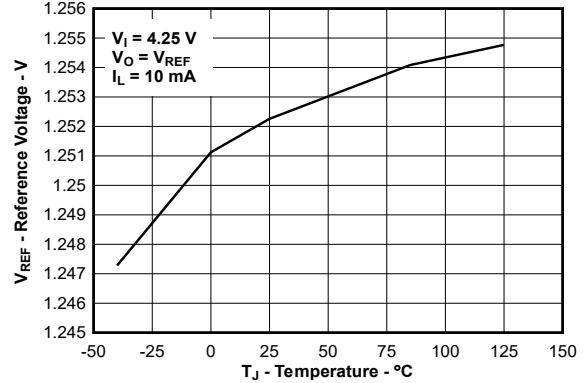
Figure 5-8. Temperature Stability vs Temperature (New Chip)
