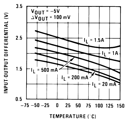
Figure 5-4. Dropout Voltage
