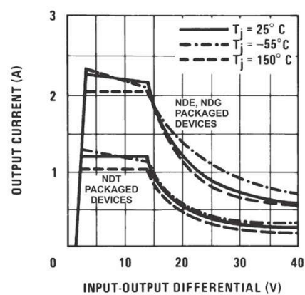
Figure 5-2. Current Limit
