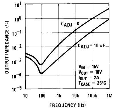
Figure 5-8. Output Impedance
