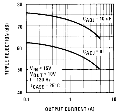
Figure 5-10. Ripple Rejection
