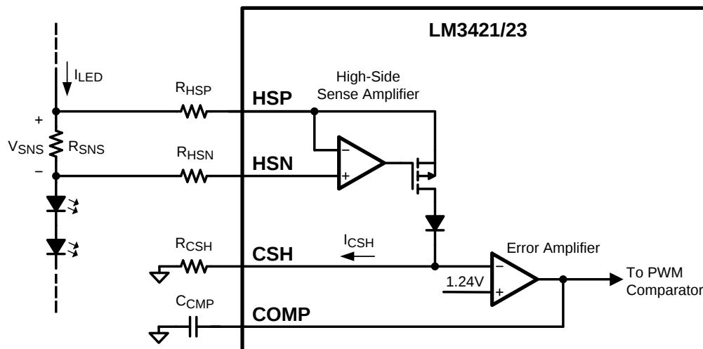
Figure 13. LED Current Sense Circuitry
