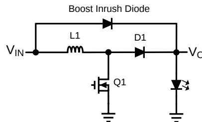
Figure 30. Boost Topology with Inrush Diode
