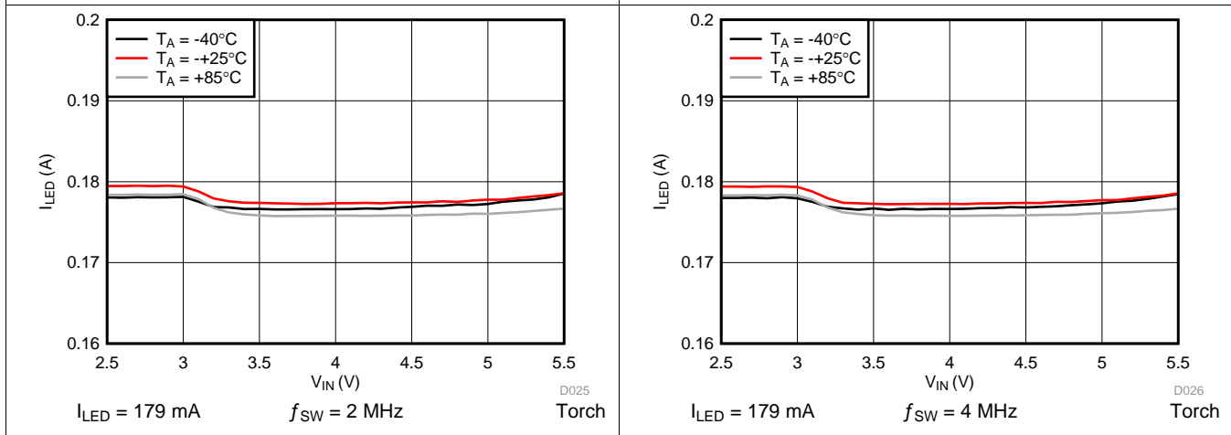
Figure 16. LED1 and LED2 Current vs Input Voltage
