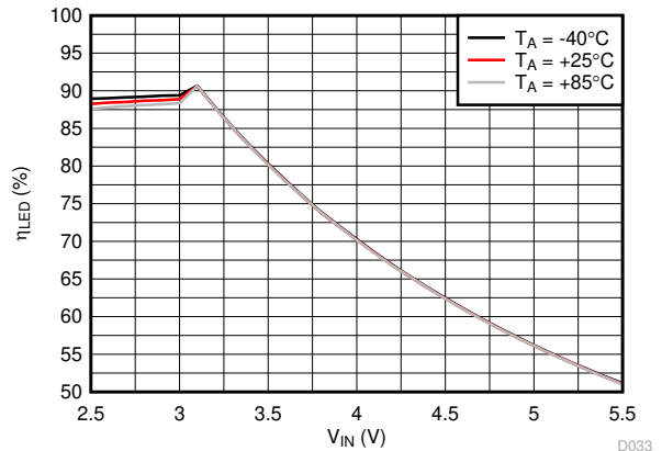
Figure 7-8. LED Efficiency vs Input Voltage
