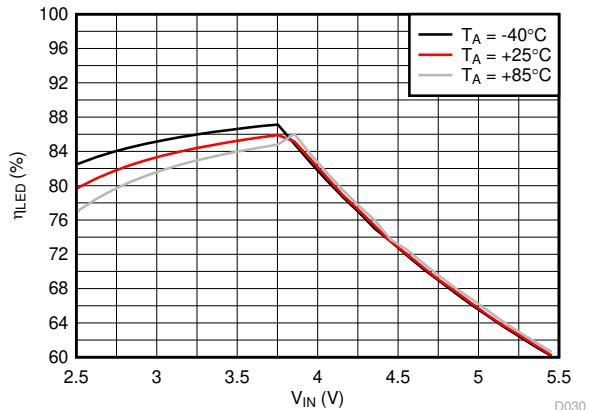
Figure 7-5. LED Efficiency vs Input Voltage
