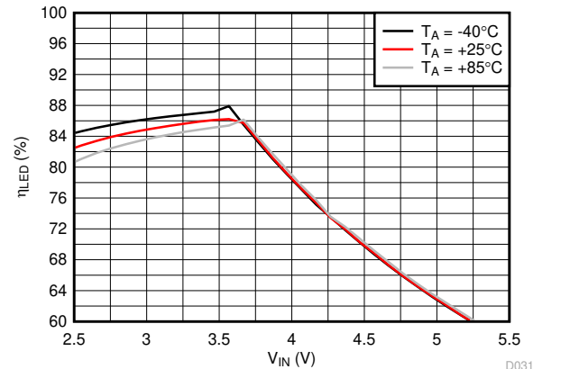
Figure 7-6. LED Efficiency vs Input Voltage
