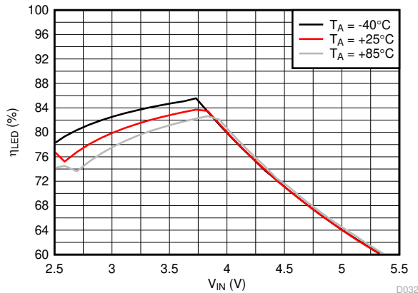
Figure 7-7. LED Efficiency vs Input Voltage
