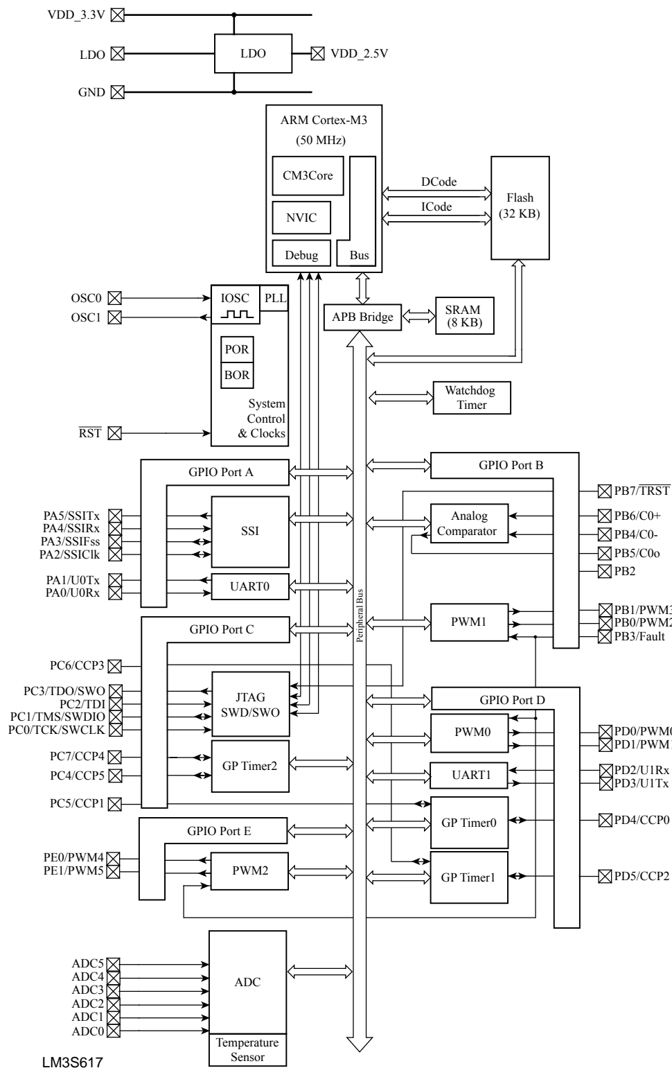
Figure 1-2. LM3S617 Controller System-Level Block Diagram
