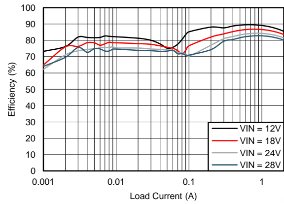
Figure 48. Efficiency
