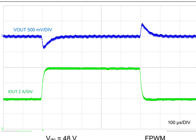
Figure 8-27. Load Transient, 4 A to 8 A
