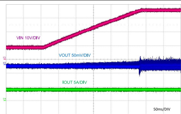
Figure 8-7. Full Load Switching
