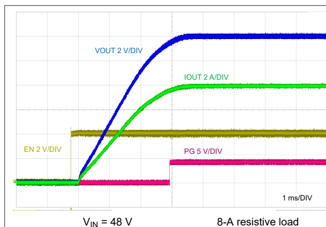
Figure 8-24. EN Start-Up Characteristic
