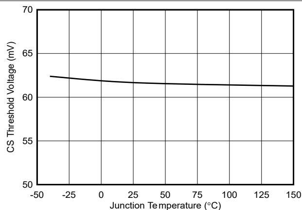
Figure 6-17. Current Sense (CS) Threshold vs Temperature
