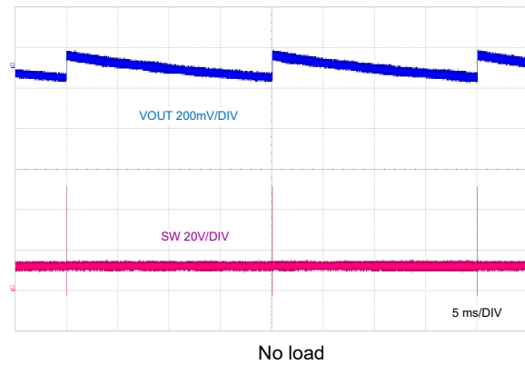
Figure 8-21. PFM Switching
