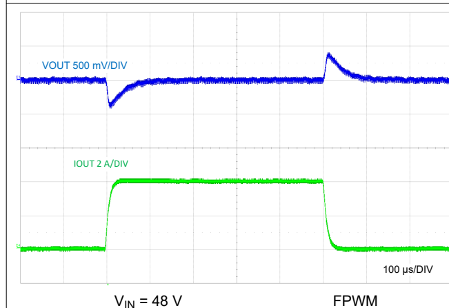
Figure 8-26. Load Transient, 0 A to 4 A
