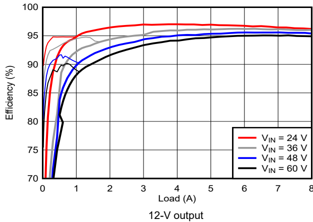
Figure 8-18. Efficiency vs I_{OUT}
