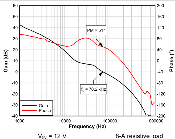
V_{IN} = 12 V 8-A resistive load Figure 8-15. Bode Plot, 5-V Output
