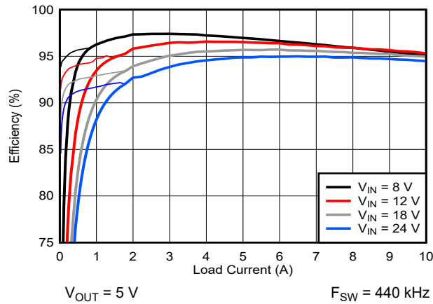
Figure 6-1. Efficiency vs Load
