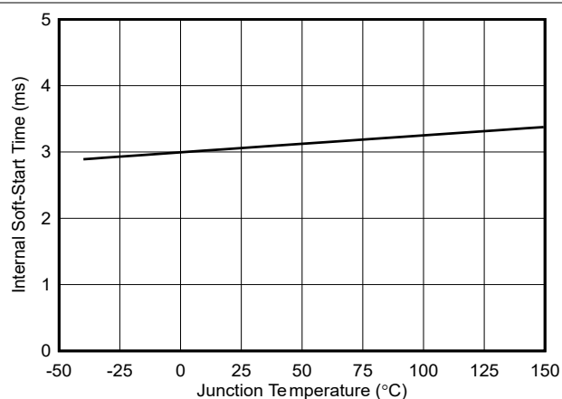
Figure 6-20. Soft-Start Time vs Temperature
