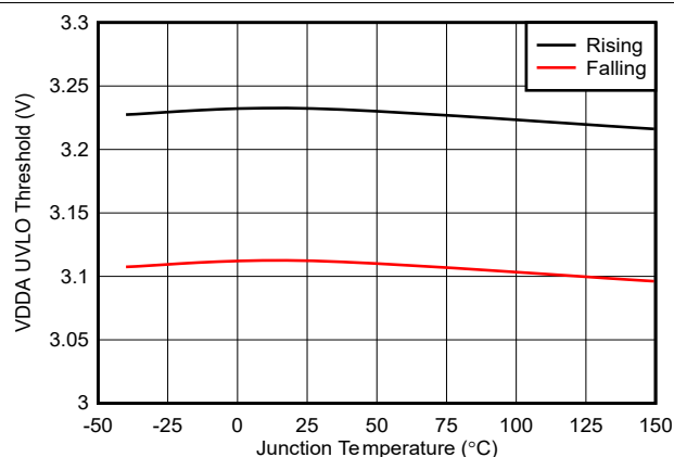
Figure 6-15. VDDA UVLO Thresholds vs Temperature
