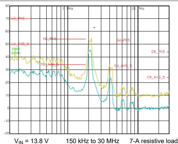
V_{IN} = 13.8 V 150 kHz to 30 MHz 7-A resistive load Figure 8-16. CISPR 25 Class 5 Conducted EMI
