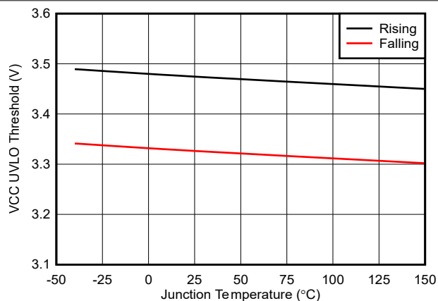
Figure 6-12. VCC UVLO Thresholds vs Temperature
