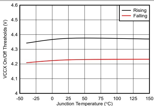
Figure 6-16. VCCX On, Off Thresholds vs Temperature
