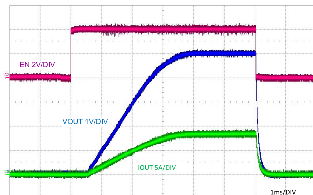
V_{IN} = 12 V 8-A resistive load Figure 8-12. ENABLE ON and OFF Characteristic
