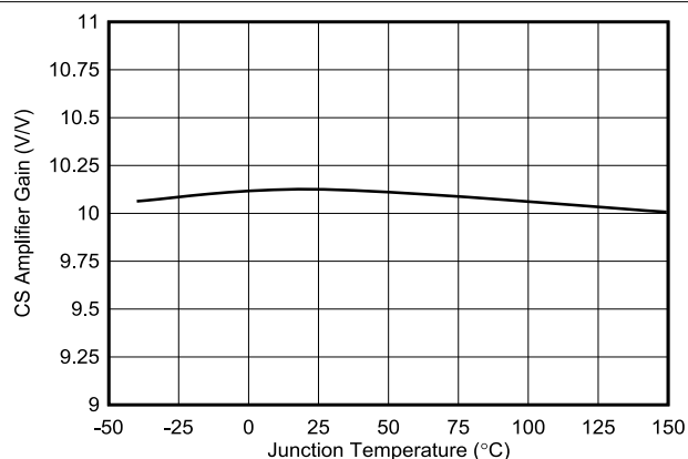
Figure 6-18. Current Sense (CS) Amplifier Gain vs Temperature
