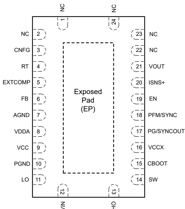
Figure 5-1. 24-Pin VQFN RGY Package With Wettable Flanks, LM5148Q1 (Top View)
