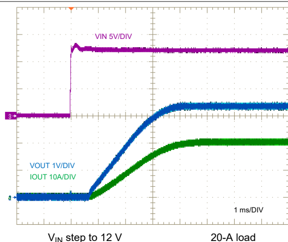
Figure 8-42. V_{IN} Start-Up Characteristic
