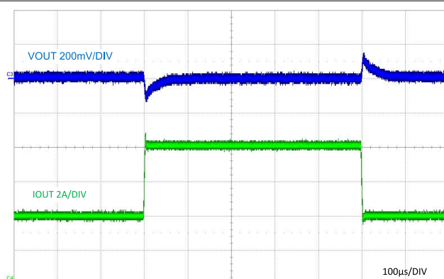
V_{IN} = 12 V FPWM Figure 8-14. Load Transient, 4 A to 8 A
