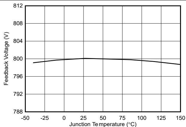
Figure 6-8. Feedback Voltage vs Temperature
