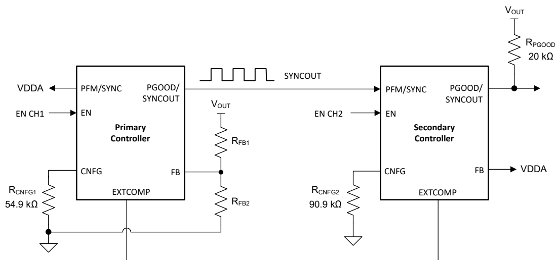
Figure 7-7. Schematic Configured for Single-Output Dual-Phase Operation
