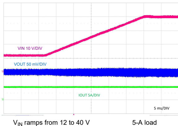
Figure 8-33. Line Transient Response to V_{IN} = 40 V
