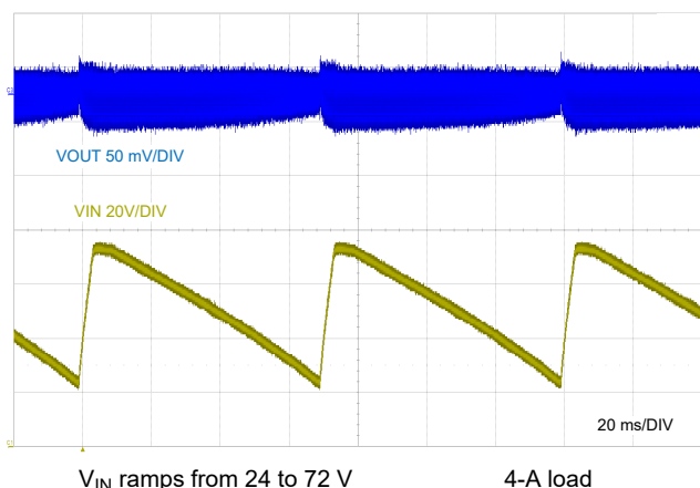
Figure 8-23. Line Transient Response to V_{IN} = 72 V
