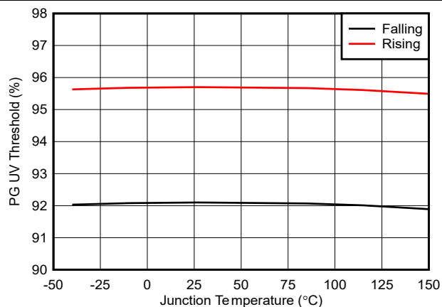
Figure 6-10. PG UV Thresholds vs Temperature
