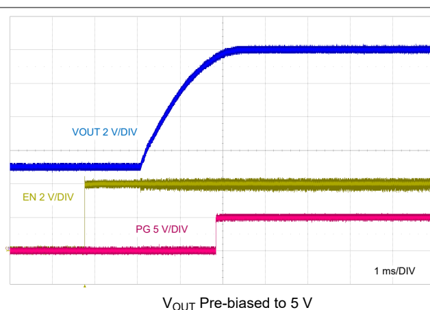
Figure 8-25. EN Start-Up Prebias Characteristic
