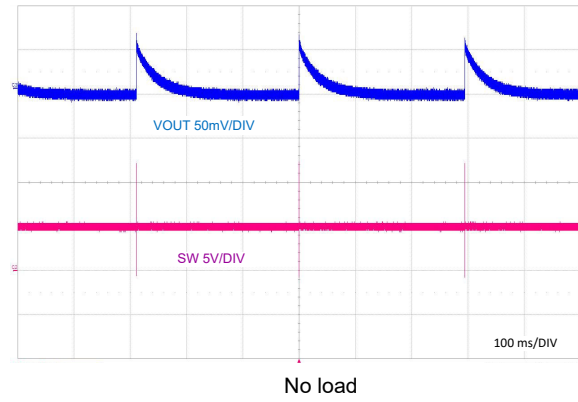
Figure 8-32. PFM Switching
