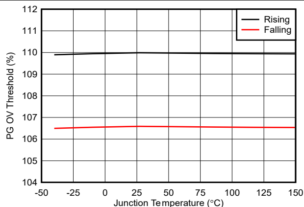
Figure 6-9. PG OV Thresholds vs Temperature
