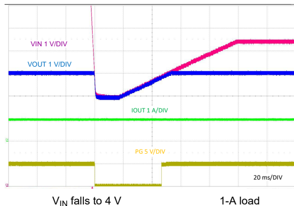
Figure 8-34. Cold-Crank Response to V_{IN} = 4 V
