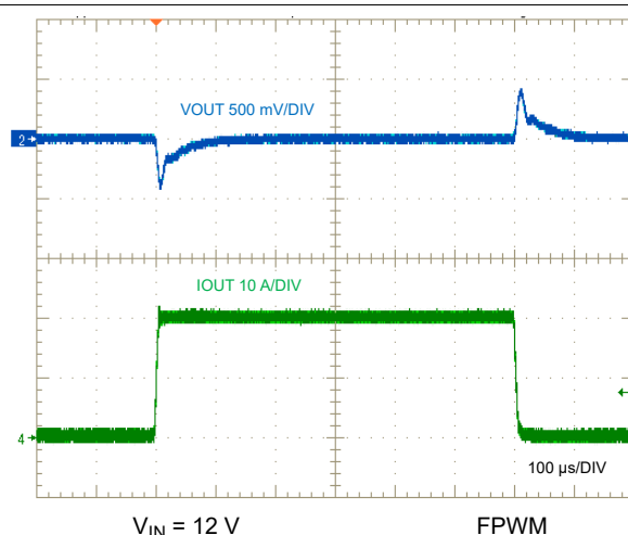
Figure 8-45. Load Transient, 0 A to 20 A
