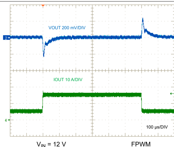
Figure 8-44. Load Transient, 5 A to 15 A
