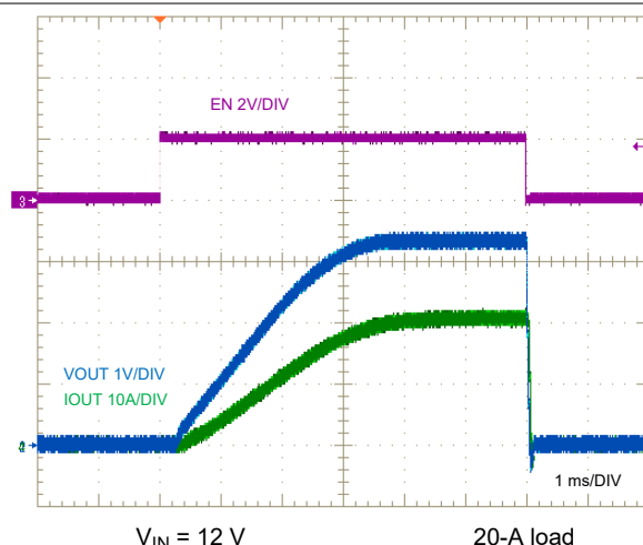
Figure 8-43. ENABLE ON and OFF Characteristic
