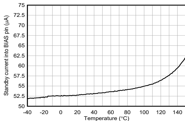
Figure 5-10. Standby Current into BIAS versus Temperature V_{(VIN)} = 3.5\text{V} , V_{(BIAS)} = 12\text{V}
