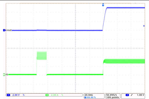
Figure 8-13. Short-Circuit Recovery
