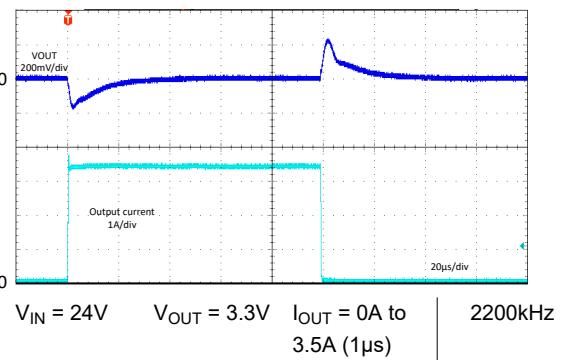
Figure 8-64. Load Transient - LM6x635 - Auto
