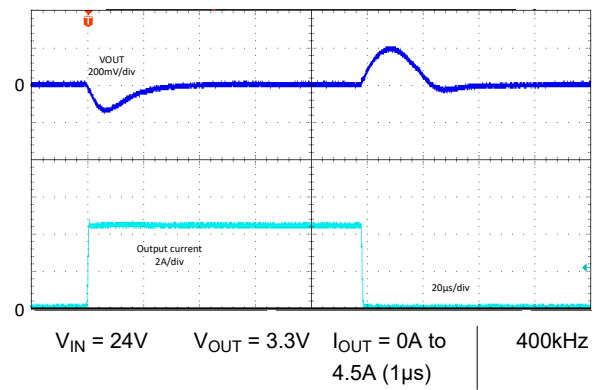
Figure 8-66. Load Transient - LM6x645 - Auto
