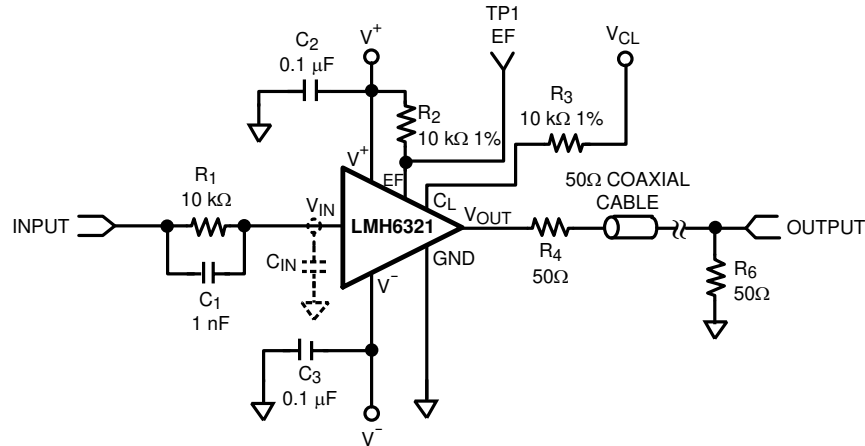
Figure 6-2. 50 Ω Coaxial Cable Driver with Dual Supplies
