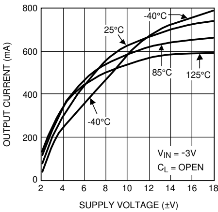
Figure 5-39. Output Short Circuit Current — Sinking vs. Supply Voltage
