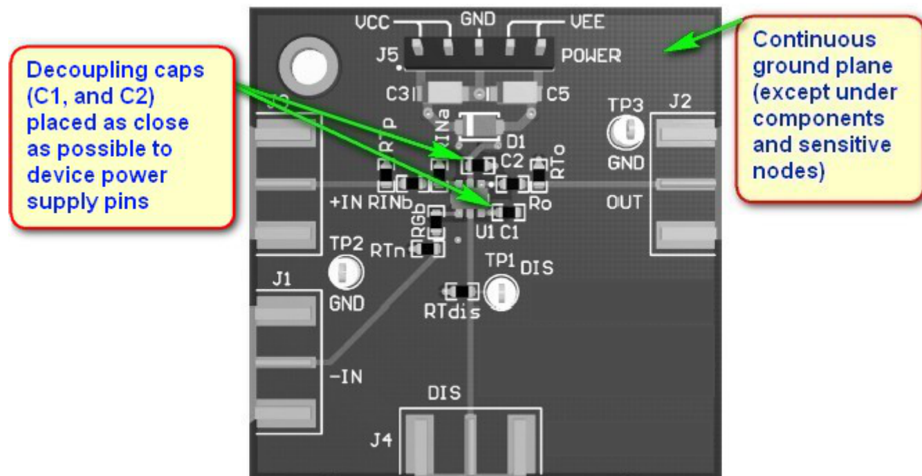
Figure 62. LMH6624 and LMH6626 EVM Board Layout Example
