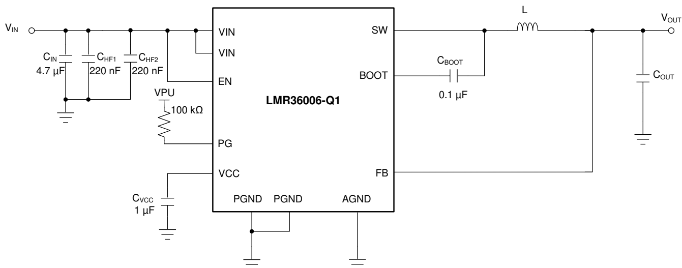
Figure 9-2. Example Applications Circuit (Fixed 3.3 V Output)
