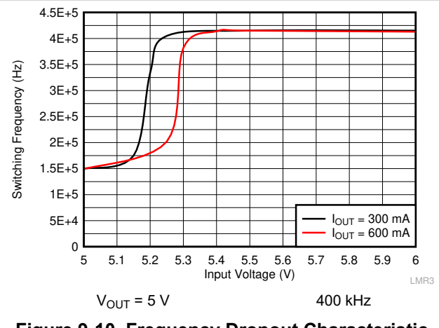
Figure 9-10. Frequency Dropout Characteristic
