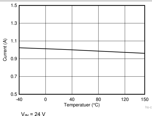
Figure 7-3. High Side Current Limit
