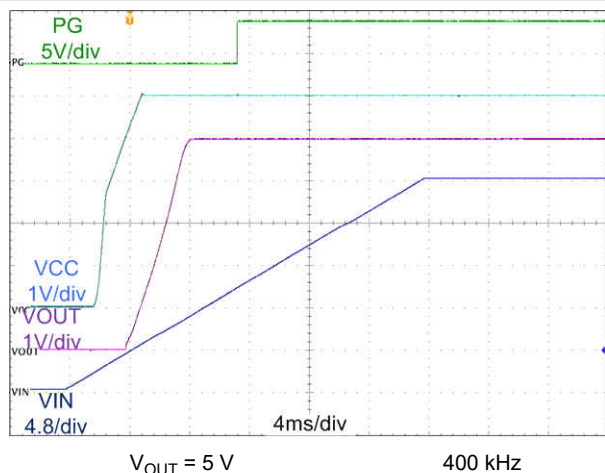
Figure 9-13. Start-Up Waveform
