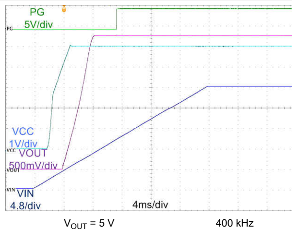
Figure 9-14. Start-Up Waveform
