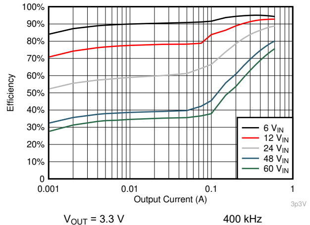
Figure 9-6. Efficiency
