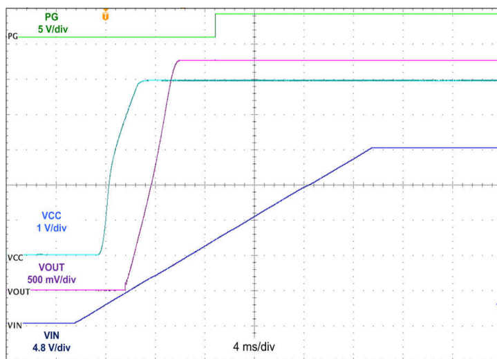
Figure 8-5. Typical Start-up Behavior V_{IN} = 24\text{ V} , V_{OUT} = 3.3\text{ V} , I_{OUT} = 0.6\text{ A}
