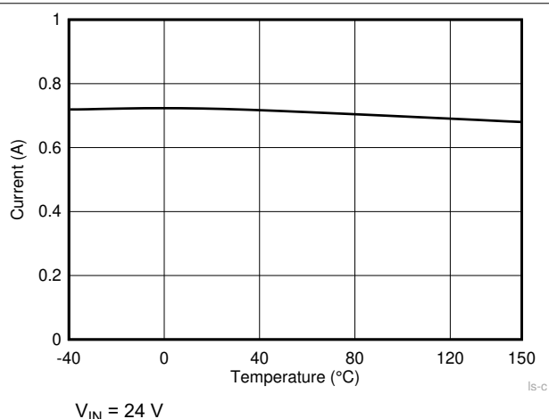
Figure 7-4. Low Side Current Limit
