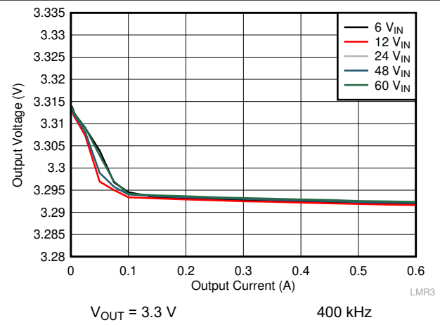
Figure 9-8. Load Regulation
