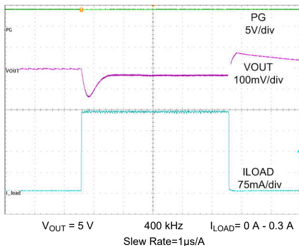
Figure 9-15. Load Transient
