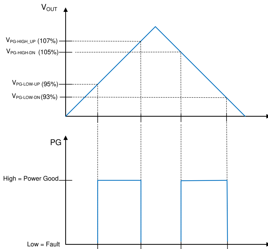
Figure 8-2. Static Power-Good Operation
