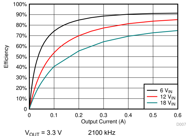
Figure 9-27. Efficiency
