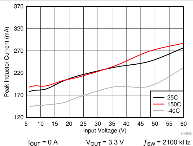
Figure 7-6. I_{PEAK-MIN}
