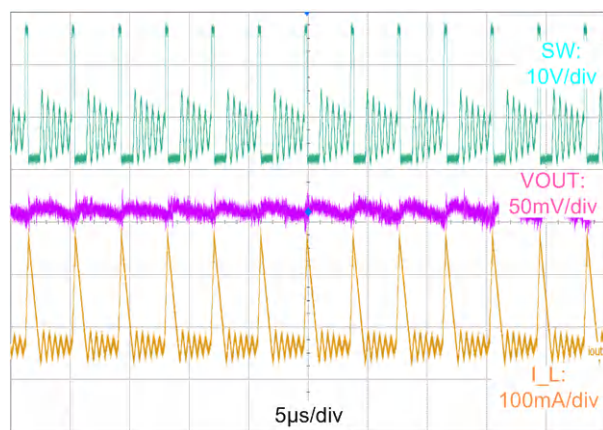
Figure 8-7. Typical PFM Switching Waveforms V_{IN} = 24\text{ V} , V_{OUT} = 5\text{ V} , I_{OUT} = 30\text{ mA}
