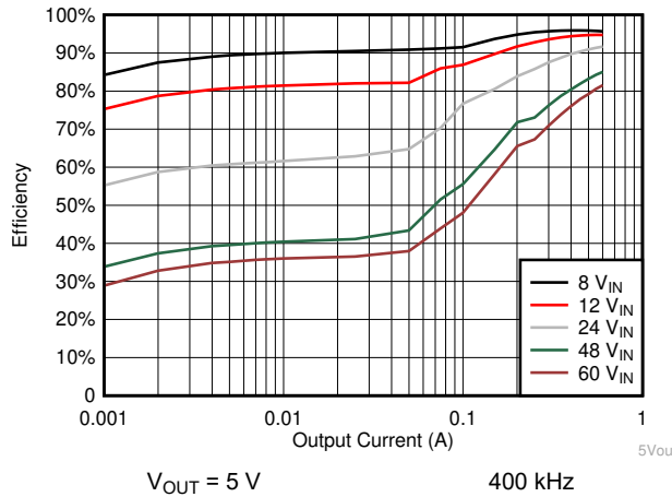
Figure 9-5. Efficiency
