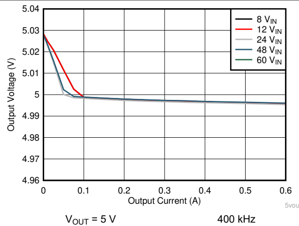
Figure 9-7. Load Regulation
