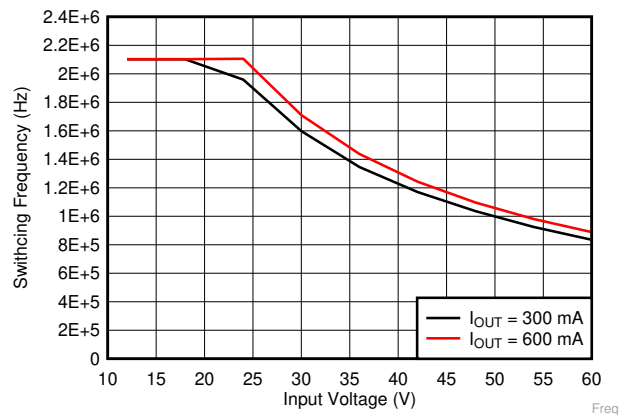
Figure 8-11. Switching Frequency vs Input Voltage V_{OUT} = 3.3\text{ V}
