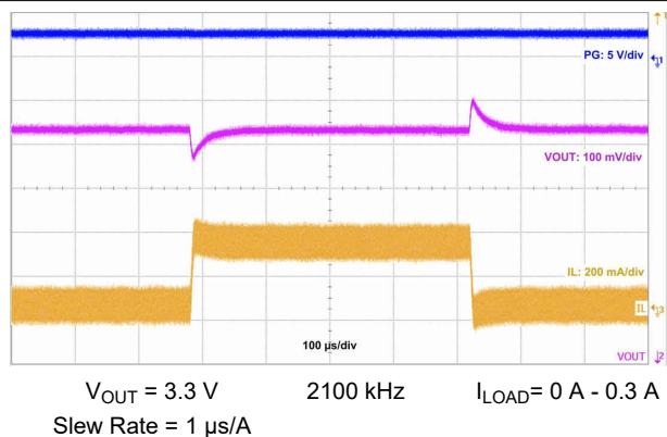
Figure 9-32. Load Transient
