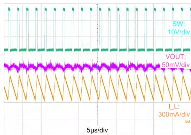
Figure 8-8. Typical PWM Switching Waveforms V_{IN} = 24\text{ V} , V_{OUT} = 5\text{ V} , I_{OUT} = 600\text{ mA} , f_s = 400\text{ kHz}
