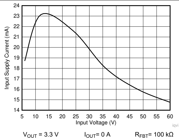
Figure 9-30. Input Supply Current
