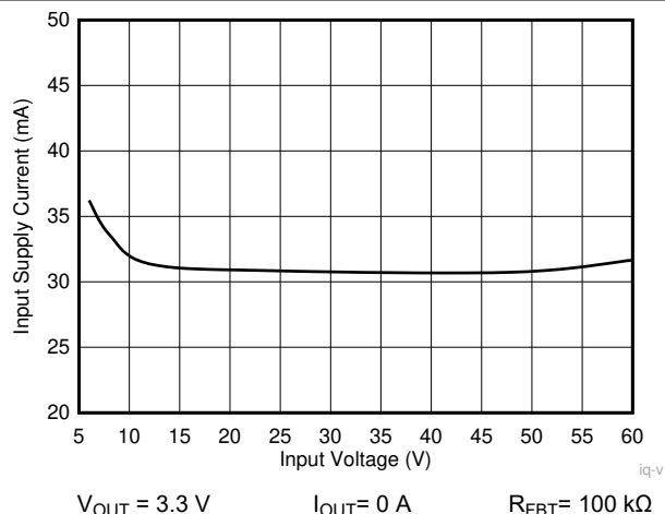
Figure 9-11. Input Supply Current
