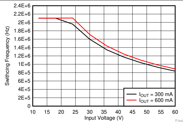
Figure 9-29. Switching Frequency vs Input Voltage
