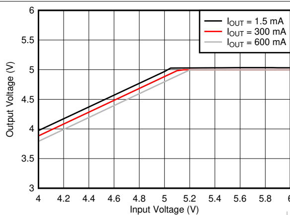
Figure 8-9. Overall Dropout Characteristic V_{OUT} = 5 V
