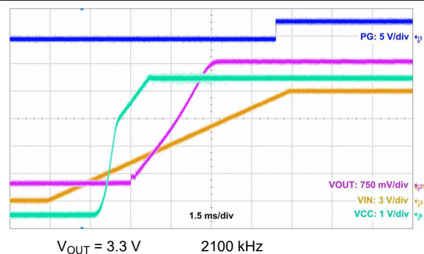
Figure 9-31. Start-Up Waveform
