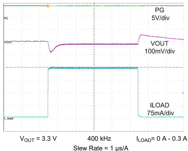
Figure 9-16. Load Transient
