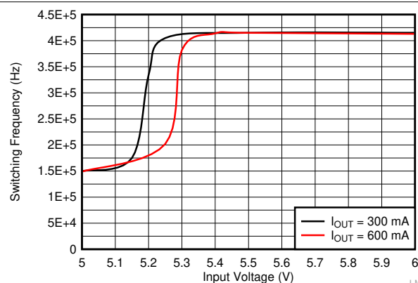
Figure 8-10. Typical f_{sw} vs Output Current f_{sw} = 400 kHz
