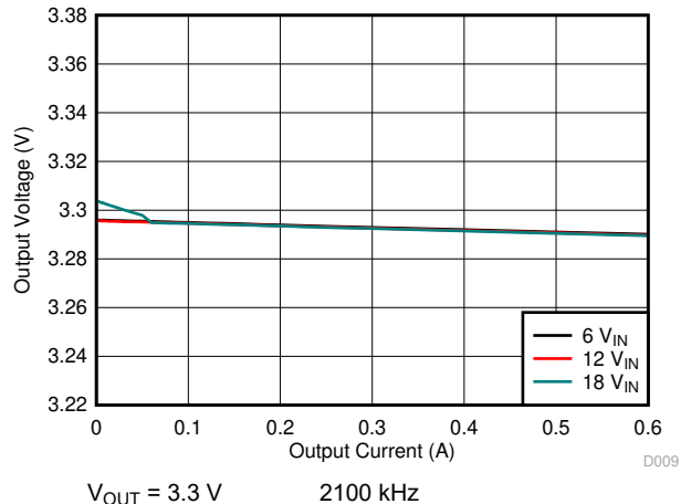
Figure 9-28. Load Regulation
