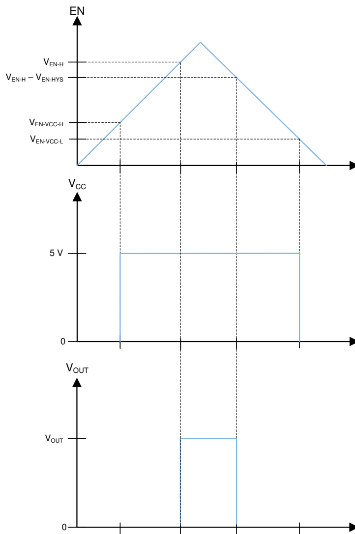
Figure 8-4. Precision Enable Behavior
