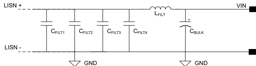
Figure 8-33. Typical Input EMI Filter Schematic
