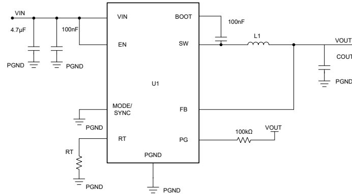
Figure 8-34. Example Application Circuit
