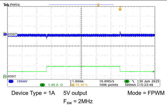
Figure 8-19. 0.5A to 1A Load Transient
